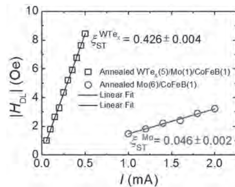
Damping-like field as a function of AC current amplitude for \text{WTe}_x(5)/\text{Mo}(1)/\text{CoFeB}(1)/\text{MgO}(2)/\text{Ta}(2) and \text{Mo}(6)/\text{CoFeB}(1)/\text{MgO}(2)/\text{Ta}(2) heterostructure, both annealed at 300^\circ\text{C} for 30 minutes.
