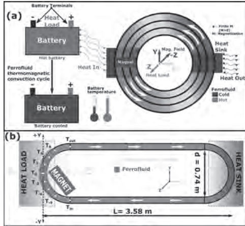
Schematics of the (a) multi-torus magnetic cooling device [1], and (b) 8 m long racetrack magnetic cooling device.
