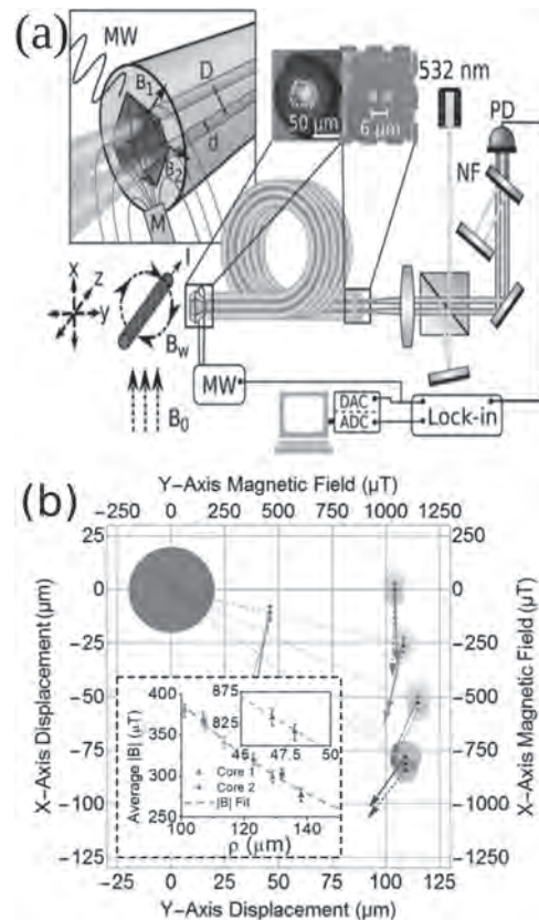
Fig. 1: (a) Experimental apparatus for the photonic crystal fiber stereomagnetometer. 4 \mu\text{m} diameter fiber cores separated by 6 \mu\text{m} (dashed red inset) interrogate NV diamond (middle inset) in microwave field (left inset). Fluorescence signal recollected by fiber imaged onto photodiode for lock-in detection. Current ( I ) generates inhomogeneous field ( B_w ) against bias field ( B_0 ) background. (b) Magnetic field vectors (colored arrows) and location of measurement points from both cores (colored circles) around wire (grey disk). Wire field magnitude as a function of radial displacement (inset figure). [5]
