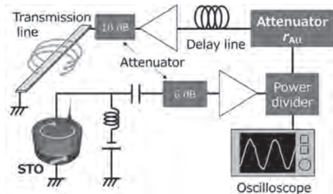
Fig. 1 Schematic illustration of self-feedback circuit. An attenuator ( r_{\text{Att}} ) controls the magnitude of the microwave field generated from the feedback current.
