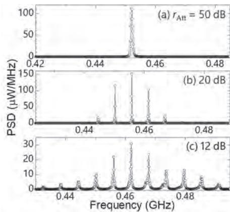
Fig. 2 Power spectrum density (PSD) of the STO for attenuation rate r_{\text{Att}} of (a)50, (b)20, and (c)12 dB, respectively.
