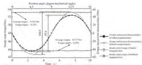
Fig. 2. Torque performance comparison of magnetic ring gear with different magnetization.
