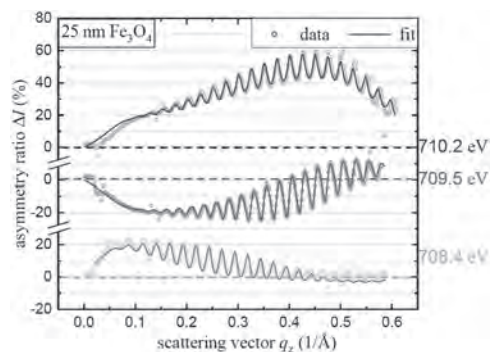
Fig. 2: XRMR data (open circles) and corresponding fits based on the algorithm introduced in [2] (solid lines) from the 25 nm thin film, recorded at the three resonant energies of the XMCD L 3 edge. Data were recorded with a magnetic field of 200 mT along the Fe 3 O 4 [001] direction at room temperature.
