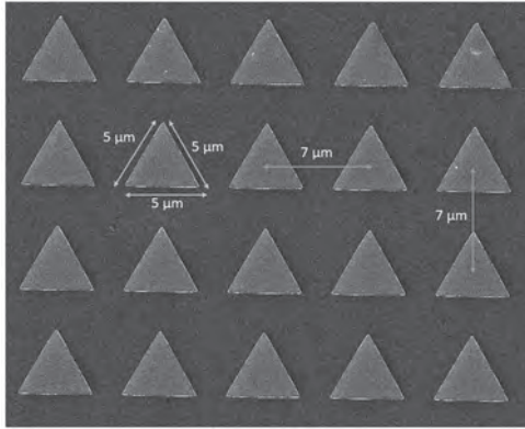
Figure 1. FESEM image of an array of equilateral triangular (vertex 5 \mu\text{m} & periodicity 7 \mu\text{m} ) fabricated using e-beam.
