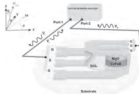
Schematic of the fabricated two port device
