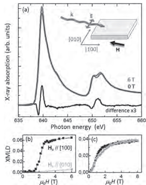
Fig.1 Spin-reorientation in antiferromagnetic \text{CuMnAs} using XMLD. (a) Mn L x-ray absorption spectra for 20 nm \text{CuMnAs} , in 0 and 6 T field, and the difference, at 200 K. The x-ray incidence k and external magnetic field H are at 15° to the sample surface. (b,c) XMLD signal vs. magnetic field for b: 20 and c: 50 nm \text{CuMnAs} films.
