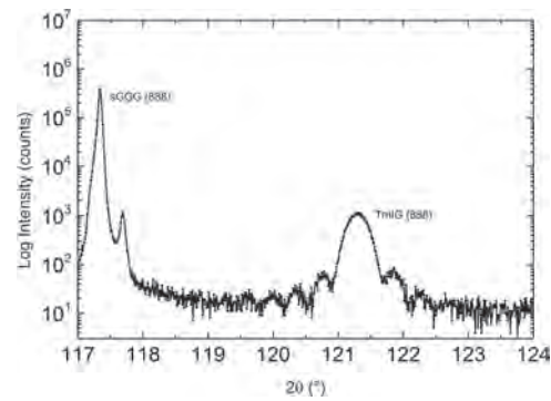
Figure 1 XRD pattern of the (888) plane for the 50nm TmIG sample
