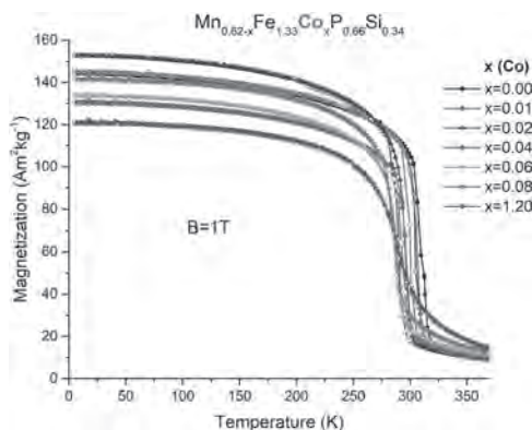
Fig. 1. Temperature dependence of the magnetization in the magnetic field of 1 T for \text{Mn}_{0.62-x}\text{Fe}_{1.33}\text{Co}_x\text{P}_{0.66}\text{Si}_{0.34} upon heating and cooling.
