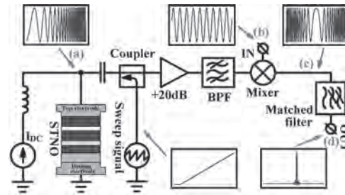
Fig. 1. Ultra-fast GHz STNO-based spectrum analyzer.
