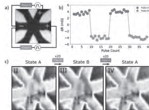
FIG1. (a) PEEM image of the 6-legged Hall cross with schematic representation of the circuit. Bright regions correspond to \alpha\text{-Fe}_2\text{O}_3 (30 nm thickness) and dark regions correspond to Pt (2 nm thickness). The Pt leads are aligned with the 3 in-plane easy axes of \text{Fe}_2\text{O}_3 . Plus and minus signs represent the connections to the two pulse generator outputs, where the minus sign indicates a connection to ground. (b) Resistance data showing switching between two states after sequential current pulses applied along either current path shown in panel a. (c) XMLD-PEEM images (4 \mu\text{m} field of view) before and after a 4 mA current pulse along the pulse A & B configurations.
