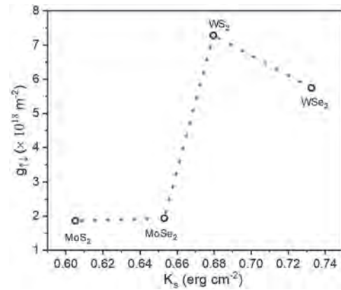
Fig.2: The plot between spin mixing conductance ( g_{\uparrow\downarrow} ) and interfacial magnetic anisotropy energy density ( K_s ) for various TMD/Py samples.
