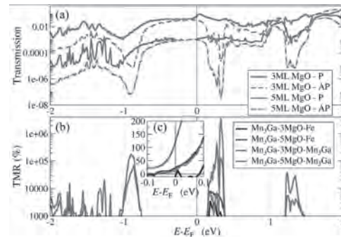
Fig. 2: Energy-resolved transmission coefficients for the different spin orientations at the interface (a) and TMR (b) for two different barrier thicknesses of \text{Mn}_3\text{Ga}/\text{MgO}/\text{Mn}_3\text{Ga} stacks, in (b) also is comparison to the Fe-polariser stack. The inset (c) is a zoom around the Fermi level.
