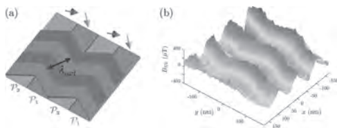
Figure: (a) Schematic antiferromagnetic spin cycloids in alternating ferroelectric domains with a surface propagation wavelength of \lambda_{\text{surf}} (b) Quantitative SNVM results on 40 nm thick epitaxially grown BiFeO 3 thin film with tensile strength of \sim +0.5\% .
