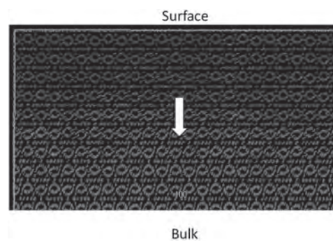
Magnetization reversal process affected by the effect of the surface magnetic anisotropy of the Nd atoms. Surface nucleation and domain growth along the c axis in the Nd magnet model.
