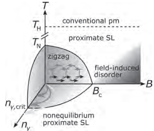
Fig. 1 A nonequilibrium dimension to \alpha -RuCl 3 's magnetic phase diagram. The (B,T)-plane sketches the equilibrium magnetic phase diagram. Photoexcited holon-doublon pairs n_y form a new nonequilibrium parameter. For small (red) to intermediate (magenta) quenches the system stays inside the zigzag ordered phase. Above a critical density n_{y,crit} a nonequilibrium proximate spin liquid state may be induced (light blue arrow).
