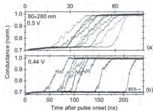
Figure 1: Conductance signatures of various STT induced switching events as a result of voltage pulses on a rectangular device. Notice the pronounced oscillations.
