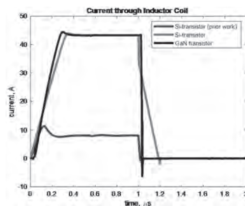
Figure 1: Comparison of current across resistor in series with inductor coil.
