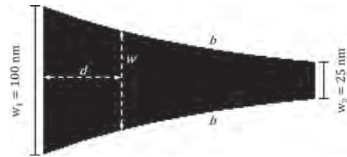
Fig. 1 Structure of the linear neuron, displaying the curvature of the neuron's sides. The curvature is of the following form: w \propto b^d , where b represents the curvature of the sides and w is the cross-sectional width of the device at any distance d from the wide end. b = 1 represents the neuron from [3].
