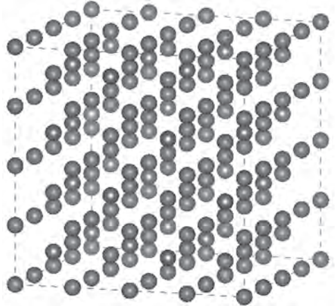
Figure 1: Crystal structure for the \text{Fe}_{79.38}\text{Ga}_{19.84}\text{Tb}_{0.78} doped
