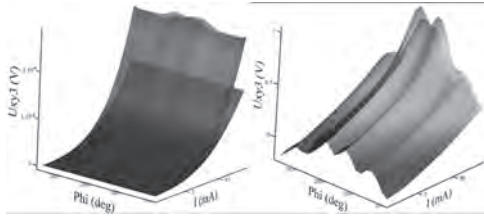
Current dependence of the third harmonic Hall voltage as a function of the direction of the in-plane applied field of 0.4 T (left). The same current and angular field dependence with background subtracted (right).
