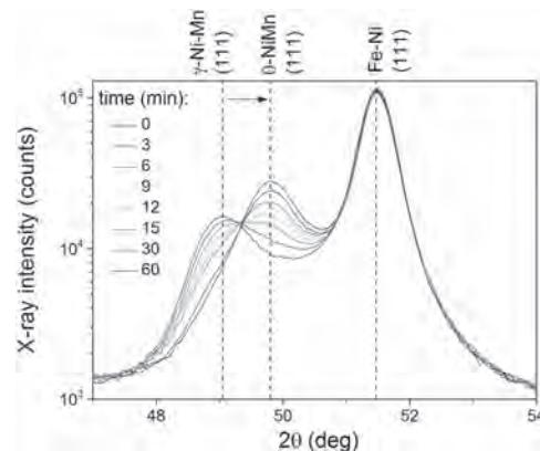
Fig. 1. Time evolution of XRD \theta -2 \theta spectra of a Fe-Ni (5 nm)/Ni 30 Mn 70 (20 nm)/Fe-Ni (40 nm) film when heated up to 300 °C. The initial \gamma -Ni-Mn under annealing transforms into \theta -NiMn, which is indicated by the shift of the (111)-peak.
