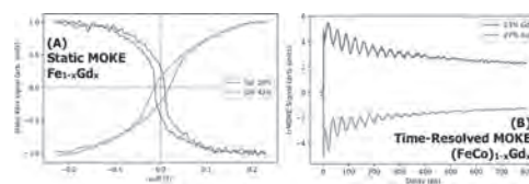
Fig. 1 (A) MOKE measurements of representative Fe 1-x Gd x samples. The reversal of the MOKE signal for the different Gd concentrations illustrates the change from Fe-dominated to Gd-dominated net moment. (B) time-resolved MOKE measurements of (FeCo) 1-x Gd x samples. The reversal of the magneto-optical signal again depicts the changeover from Fe- to Gd-dominated net moment, along with ultrafast demagnetization, followed by the onset of precession oscillations and a return to equilibrium.
