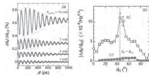
Fig. 1 (a) The TRMOKE results at the critical magnetic field angle \theta_{H,c} , with different pump power P_{\text{pump}} = 3, 5, 7 , and 10 mW. At P_{\text{pump}} > 5 mW, temporal amplification of the magnetization precession was observed (dashed curves). (b) The \theta_H dependence of FFT power density for acoustic (AC) and optical (OP) mode. Dashed line shows the \theta_{H,c} where the peak of the AC mode remarkably enhanced.
