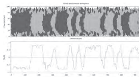
HAMR write/read simulation of a pseudorandom bit sequence performed using MARS via the LLB and kMC solvers. Upper part shows magnetisation of the grains. The lower part shows the obtained readback signal.
