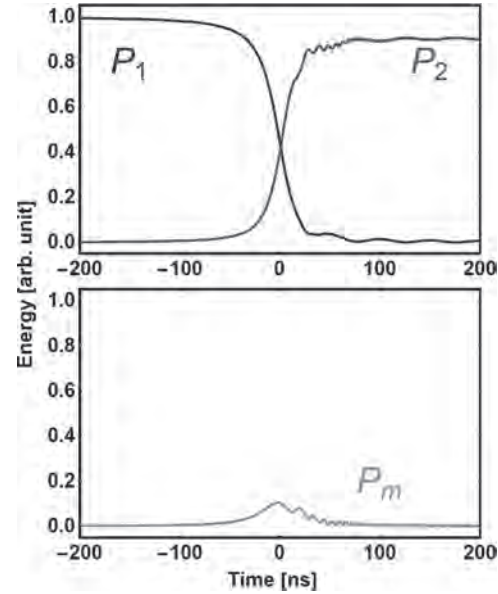
Fig. 1. Temporal profiles of populations of two superconducting resonators P_{1,2} (top) coupled to magnetic resonator P_m (bottom) during the fast (ramp rate \rho/2\pi = 2.5 MHz/ns) tuning process of the magnetic resonance frequency.
