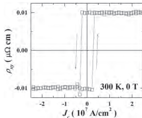
Hall resistance vs. current density for \text{Mn}_3\text{GaN/Pt} bilayers. (300 K, 0 T)
