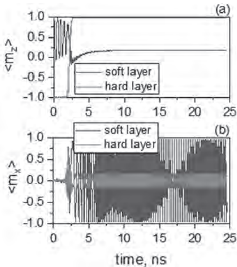
Fig. 2. (a) Average normalized magnetization m_z and (b) m_x vs. time for J_{AF}=-0.15 erg/cm². An applied current density was J=20 MA/cm².
