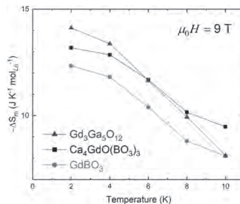
Fig. 1: Magnetic entropy change per mole of lanthanide ion at 9 T: comparison between \text{Ca}_4\text{GdO}(\text{BO}_3)_3 , \text{GdBO}_3 and the standard magnetocaloric material \text{Gd}_3\text{Ga}_5\text{O}_{12} (GGG).
