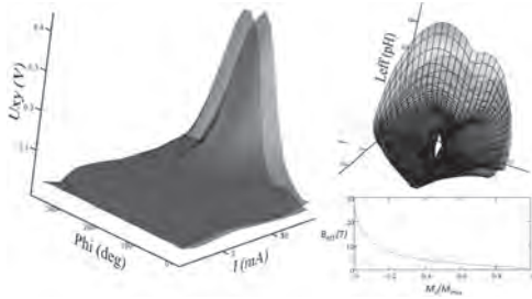
Scaled third harmonic Hall voltage as a function of current and the inplane orientation of \mu_0|H| = 0.4 T, with background subtracted (left). Spin-orbit torque induction for various in-plane applied field directions and various currents (top right). B_{\text{eff}}(m_z/m) (bottom right).
