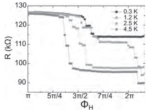
Fig.2: TMR experiments where the magnetic field is rotated in the in-plane direction of the samples, with |H|=70 Oe, for different temperatures, showing how new stable magnetic configurations arise under T=2 K. The changes in resistance values correspond to different magnetic states of the spin-valve: antiparallel (around 125 kΩ), 135 degrees (for the two low-temperature measurements, 115 kΩ), perpendicular in plane (100 kΩ) and parallel (90 kΩ, in the 4.5 K experiment).
