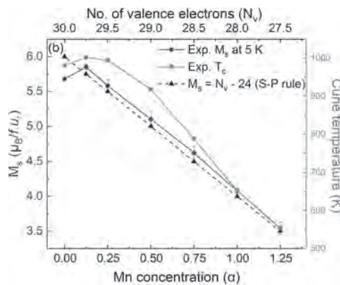
(b) Magnetic moment and Curie temperature variation with Mn concentration in (\text{Co}_{2-x}\text{Mn}_x)\text{FeGe} series.
