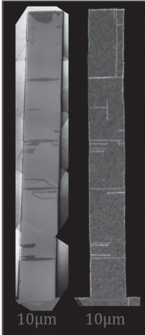
Fig. 1: AF domain structure and correlation to microtwin defects in a patterned 80μm x 10μm sized CuMnAs stripe. Left: AF domain structure imaged in XMLD-PEEM. The double-headed red arrows indicate the local spin axes. Right: Scanning X-ray diffraction map of the same bar showing the distribution of line-defects. The image axes are aligned with the CuMnAs [110] and [1-10] crystalline axes.
