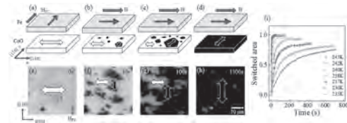
Figure 1. (a) Schematics of spin configurations in Fe/CoO bilayer after field cooling. (b)-(d) Schematics of time-dependent CoO AFM domain switching. (e)-(h) Time-dependent AFM domain evolution of Fe/CoO bilayer under a fixed field. (i) Temperature dependence of switched area of CoO domain as a function of time under a fixed field.
