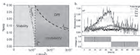
Fig. 1 a. STT efficiency dependence of the working regions. b. Resistance variation due to a train of pulses as in the bottom panel.
