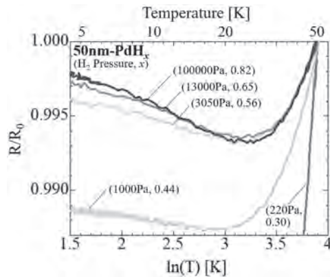
Fig. 1 Temperature dependence of resistance for 50-nm-thick PdH x .
