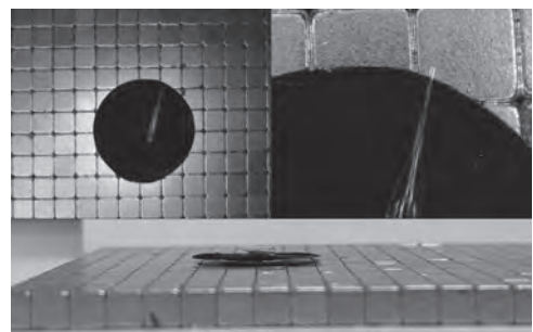
Fig. 2. Photographs of a micropipette resting on top of a diamagnetically levitated 15mm \Phi PyG sample.
