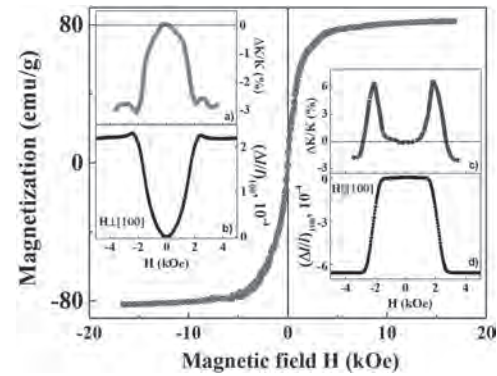
Field dependences of magnetization of CoFe 2 O 4 at H||[100]. In the insets, ones of the magnetostriction (\Delta l/l)_{00} and the magnetoabsorption \Delta K/K at \lambda = 2.7 \mu\text{m} .
