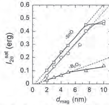
Fig. 1. Dependence of the torque coefficient of twofold components ( I_{20} ) for typical granular films with B_2O_3 , SnO, and C on the film thickness ( d_{\text{mag}} ).
