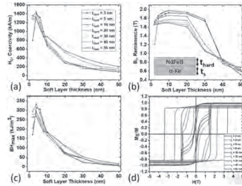
Fig. 1: Change of (a) H_c , (b) B_r , (c) (BH)_{\max} with \alpha\text{-Fe} layer thickness t , for different \text{Nd}_2\text{Fe}_{14}\text{B} layer thickness t_{\text{hard}} . (d) M-H hysteresis loops for t_{\text{hard}} = 10 nm with varying soft layer thickness.
