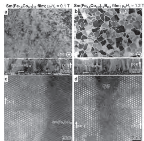
Fig. 1. Plane-view (top) and cross-sectional (bottom) BF-TEM images of (a) \text{Sm}(\text{Fe}_{0.8}\text{Co}_{0.2})_{12} and (b) \text{Sm}(\text{Fe}_{0.8}\text{Co}_{0.2})_{12}\text{B}_{0.5} films. HAADF-STEM images obtained from the cross-sectional view of (c) \text{Sm}(\text{Fe}_{0.8}\text{Co}_{0.2})_{12} and (d) \text{Sm}(\text{Fe}_{0.8}\text{Co}_{0.2})_{12}\text{B}_{0.5} films.
