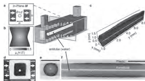
Wall-less magnetic confinement in a fluidic channel. Centre : exploded view, where permanent magnets (red, blue) in an in-plane quadrupolar configuration create a low-field zone at the centre a , where an antitube of water (yellow) is stabilized inside an immiscible magnetic liquid; b contour plot of the magnetic field; c synchrotron X-ray tomographic reconstruction of a water antitube (yellow) with diameter 81 \mu\text{m} surrounded by ferrofluid (blue); d optical end-view of a water antitube in ferrofluid; e X-ray end-view cross-section from tomographic data at y = 4 \text{ mm} ; and f X-ray side-view cross-section from tomographic data at x = 1 \text{ mm} . Scale bars (black/white) are 2 mm.
