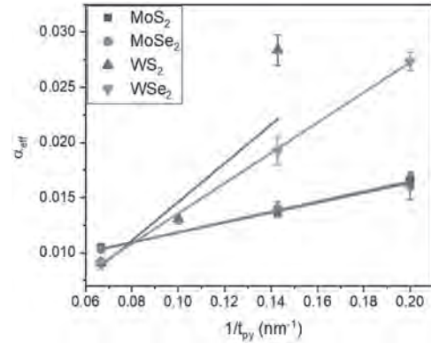
Fig.1: Gilbert damping parameter ( \alpha_{\text{eff}} ) vs. inverse of Py thickness to determine spin mixing conductance ( g_{\uparrow\downarrow} ).
