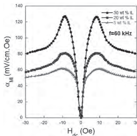
MI coefficients of the fabricated structures as a function of the applied DC magnetic field at 60 kHz
