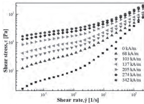
Figure 2. Shear stress and of rGO/CoFe 2 O 4 based MR fluid as a function of shear rate under various magnetic field strengths
