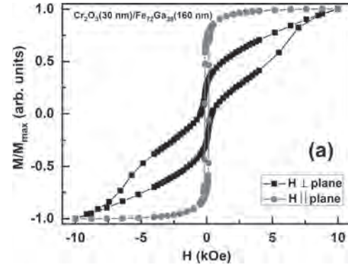
(a) Perpendicular (■) and in-plane (●) room temperature hysteresis loops recorded after a field-cooling process with the applied magnetic field perpendicular to the sample plane of 90 Oe (a) \text{Cr}_2\text{O}_3(30 \text{ nm})/\text{Fe}_{72}\text{Ga}_{28}(160 \text{ nm}) .
