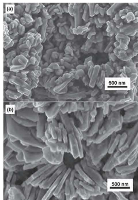
Fig.1. Scanning electron micrographs of barium hexaferrite platelets synthesized in the presence of (a) KBr and (b) K 2 CO 3
