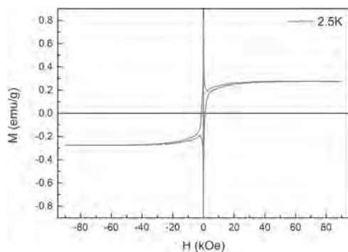
Fig. 1: Hysteresis loop of annealed \text{Ni}_2\text{NbSn} Heusler alloy at 2.5K
