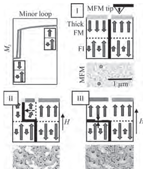
The thicker FM layer switches irreversibly as indicated by the presence of hysteresis in the M - H minor loop. I-III show schematically the reversal process starting from the demagnetized state. The corresponding in-field MFM images are displayed underneath.
