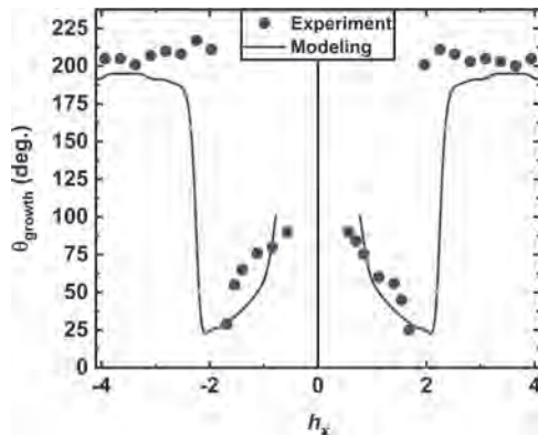
Figure 2: The favored growth direction \theta_{\text{growth}} (relative to the in-plane field direction) of domains in a [\text{Co}/\text{Ni}/\text{Pt}]_3 sample as a function of reduced in-plane field strength h_x as observed experimentally and compared to a steady-state dynamic-stiffness-creep model.
