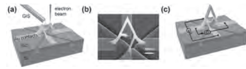
Fig.1 Direct fabrication and measurement of the Co nanobridge
