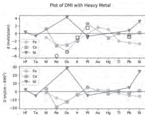
Plots of Dzyaloshinskii-Moriya interaction (DMI) for a series of HM/FM bilayers. Our DMI results are plotted with filled markers, whereas corresponding DMI values in literature are plotted using unfilled black markers. Circles represent Fe, squares represent Co and triangles represent Ni. The unit of D is \text{mJ}/(\text{m-BM})^2 , where BM is the Bohr magneton.
