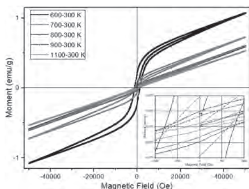
Fig.2. Room temperature measurements of magnetization vs magnetic field for \text{LaCo}_{0.5}\text{Fe}_{0.5}\text{O}_3 sintered at different temperatures.
