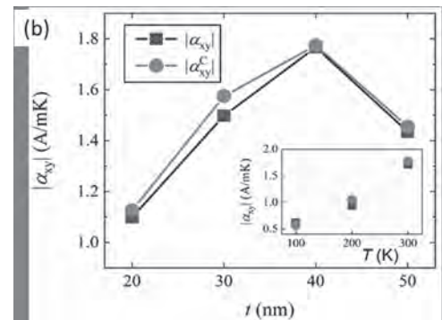
The measured and calculated anomalous Nernst conductivity is in excellent agreement in the whole sample series suggesting that the Mott relation is applicable to the \text{Co}_2\text{MnGa} Weyl semimetal.
