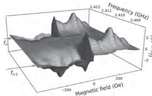
Fig.2. 3D image of voltage U_{ISHE} in Pt layer versus frequency and field. The red arrows indicate the resonant frequencies of HBAR.
