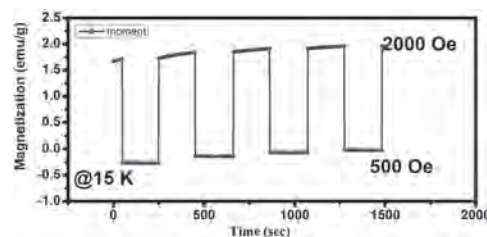
Fig.1 Magnetic switching behavior of \text{GdMn}_{1-x}\text{Cr}_x\text{O}_3 perovskite
