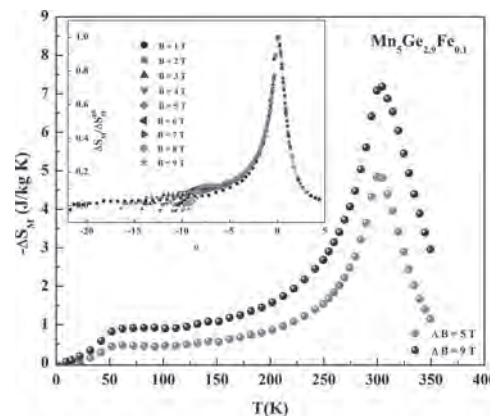
Fig. 1: Main Panel: The magnetic entropy change (MCE) of \text{Mn}_5\text{Ge}_{2.9}\text{Fe}_{0.1} compound. Inset: Universal curve demonstrating the second order nature of the compound.
