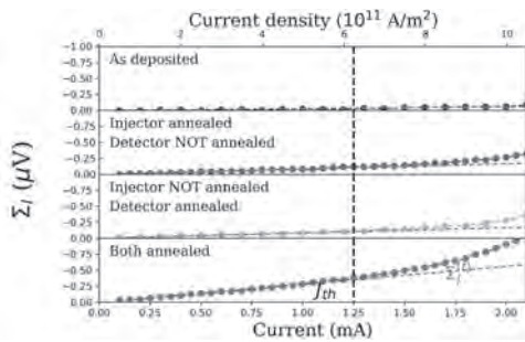
Fig.2: Non-local SOT related magnon transport signals ( \Sigma ). The first panel (top) shows the signal directly after the nanofabrication. The second and the third panel represent the signals with one-hour annealing at either the injector strip or the detector strip. In the last panel (bottom), both the injector and detector are annealed.
