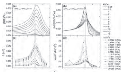
Figure 2. (a,b) The magnetoresistance versus reduced temperature t , with magnetic field H applied along the magnetic easy axis [1-10]; (c,d) Plots of \delta(m^2) vs. t and \delta(m^2)/h vs. t obtained from magnetometry measurement, where \delta(m^2) = m^2(h) - m^2(0) m is the reduced magnetization and h is the reduced field.
