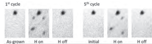
Figure 1 Spin-polarized low energy electron microscopy image sequence of magnetic Ni/Co bilayer with out-of-plane sensitivity (black + M_z , white - M_z ), capturing the reversible creation/ annihilation of skyrmions during cycles of hydrogen chemisorption/desorption, which is attributed to the hydrogen-induced magnetic anisotropy. The field of view is 1.5 \mu\text{m} \times 2.1 \mu\text{m} .
