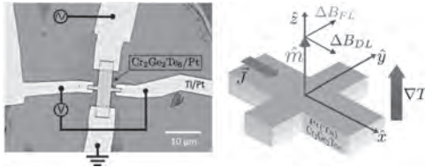
(left) Optical image of \text{Cr}_2\text{Ge}_2\text{Te}_6/\text{Pt} heterostructure patterned into a Hall bar geometry for transport measurements. (right) Schematic illustrating the orientation of effective fields due to current-induced damping like torque \Delta B_{DL} and field-like torque \Delta B_{FL} . The injected current also generates an out-of-plane thermal gradient resulting in large magnetothermal signals.
