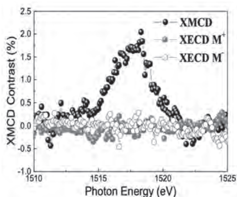
XMCD contrasts of the remnant magnetization (measured under zero magnetic field after application of \pm 18 kOe magnetic field) and X-ray electric circular dichroism (XECD) contrasts between FE polarization up and down under magnetic field +18 kOe (XECD M^+ ) and -18 kOe (XECD M^- ) at \text{Yb } M_5 edge.
