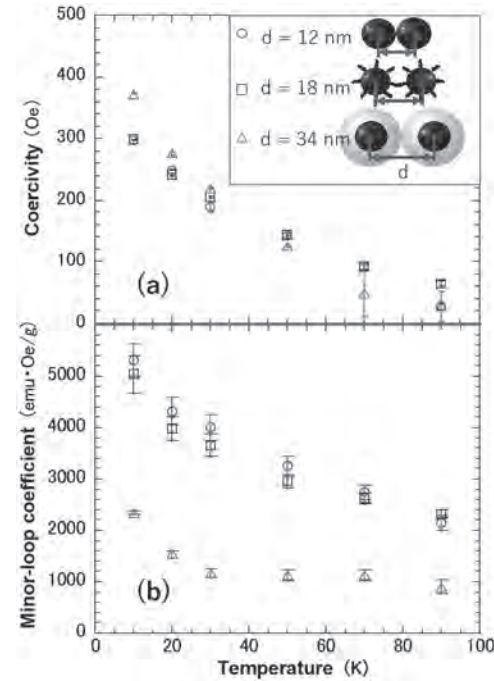
(a) Coercivity and (b) minor-loop coefficient, as a function of temperature. The inset in (a) shows a schematic diagram of each sample.
