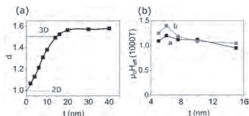
Fig.2 (a) Power law exponent d in the dependence \langle \phi^2 \rangle = CH^{d-2} of the average square of the angle between the magnetization and external field, vs Py film thickness, determined from micromagnetic simulations. Dashed lines show the analytical results for 2D and 3D systems. (b) Magnitude of the effective random exchange field in Py/CoO bilayer vs Py thickness, determined from the two branches of the hysteresis loop for the field aligned with the cooling field.
