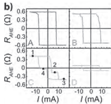
Fig. 1b) Current driven SOT switching curves at specific doses chose from a) under a bias field of \mu_0 H_x = 150 \text{ mT} .
