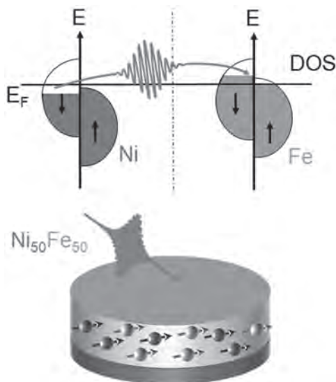
Illustration of the optically induced spin transfer process in a Fe-Ni alloy
