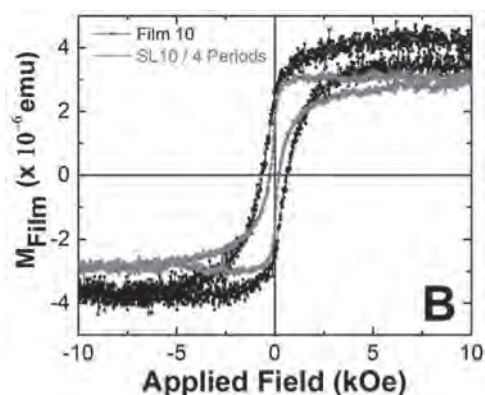
Magnetic hysteresis loops at 1.8 K shows a different magnetic response of 1D iron chains based in FePc films and FePc/ \text{H}_2\text{Pc} SLs
