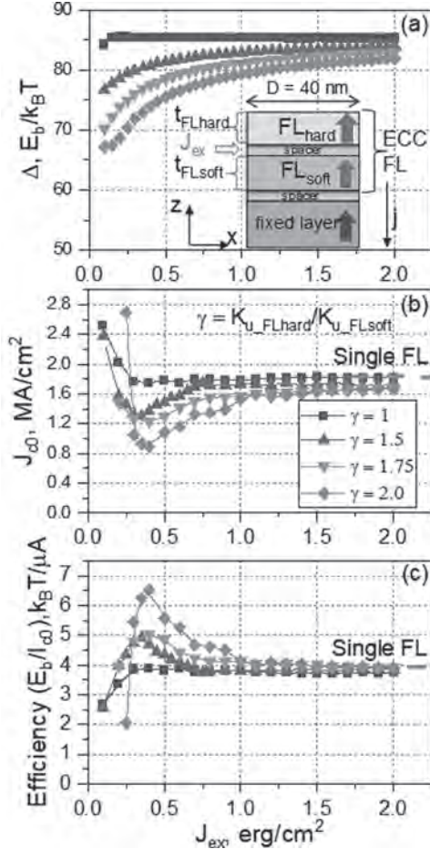
Fig.1. (a) \Delta (b) J_{c0} (c) Efficiency vs. exchange coupling constant J_{ex} with M_{sFLhard} = M_{sFLsoft} = 960 emu/cc, K_{uFLhard}/K_{uFLsoft} = \gamma , A_{ex} = 10^{-6} erg/cm, \alpha = 0.008 , t_{FLhard} = t_{FLsoft} = 1.2 nm, t_{spacer} = 1.0 nm
