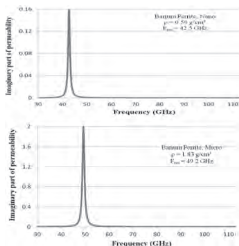
Fig 2. Imaginary parts of permeability for Barium nano-ferrite powder and micro-ferrite powder measured in the millimeter wave frequency range.
