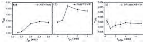
Figure 1 (a) Variation of \alpha_{\text{eff}} with thickness of top-Pt layer, (b) Variation of \alpha_{\text{eff}} with thickness of underneath-Pt layer, (c) Variation of \alpha_{\text{eff}} with thickness of underneath-IrMn layer.
