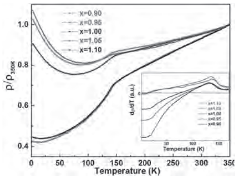
FIG. 2. The temperature-dependent relative resistivity \rho/\rho_{350K} for \text{SrRu}_x\text{O}_3 ( 0.9 \leq x \leq 1.1 ). The inset shows the dp/dT vs the Temperature curve.
