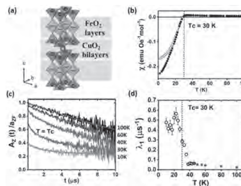
Figure 1. (a) Crystal structure of the \text{FeSr}_2\text{YCu}_2\text{O}_{7+\delta} compounds, comprising \text{CuO}_2\text{-Y-CuO}_2 bilayers stacked between \text{SrO-FeO}_{1+\delta}\text{-SrO} blocks. (b) Magnetic susceptibility for the \text{FeSr}_2\text{YCu}_2\text{O}_{7.56} sample showing the superconducting transition at T_c=30 K. (c) ZF- \mu\text{SR} spectra and (d) the derived temperature dependence of the relaxation rate for the same sample, evidencing the onset of the magnetic interactions at T \sim T_c .
