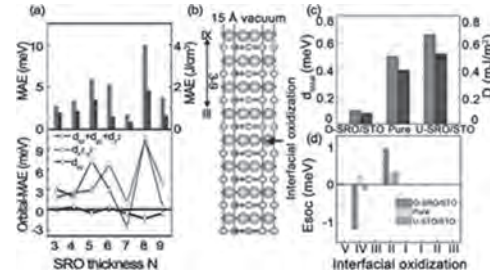
Magnetic anisotropy energy and Dzyaloshinskii-Moriya interaction of SRO/STO heterostructures with different SRO ALs and interfacial oxidations.
