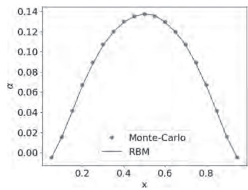
Fig. 1. Warren-Cowley parameter for binary alloy.
