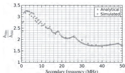
Fig. 1. Threshold field, h_{th} , with secondary ( h_{th0} : without) w.r.t primary signal of 6 GHz is determined as the secondary signal frequency is varied.
