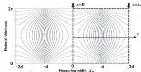
Eddy-current distribution in the magnetic material
