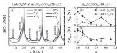
Fig. 1. (a) Operando synchrotron X-ray diffraction from a 28-unit-cell-thick \text{La}_{0.5}\text{Sr}_{0.5}\text{CoO}_{3-\delta} film on \text{LaAlO}_3 at various gate biases at 150 K. Sr-doping (x) dependence of (b) the threshold voltage ( V_{th} ) for the P to BM transition and (c) the window of reversibility ( \Delta V_{rev} ) for 28-unit-cell \text{La}_{1-x}\text{Sr}_x\text{CoO}_{3-\delta} films on \text{LaAlO}_3 and LSAT substrates. \epsilon_{xx} denotes in-plane biaxial strain.
