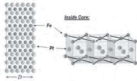
Fig.1 Illustration of atomic structure in a L1_0 ordered FePt grain.
