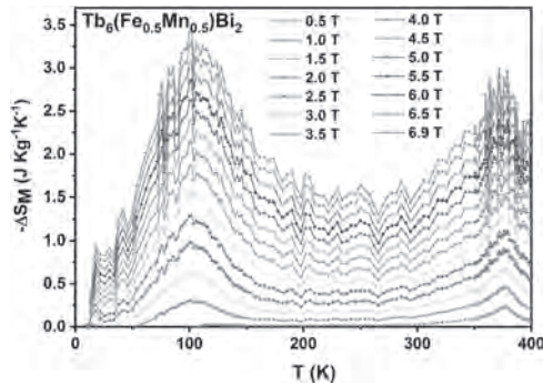
Fig. 1: DMCE for \text{Tb}_6\text{Fe}_{0.5}\text{Mn}_{0.5}\text{Bi}_2
