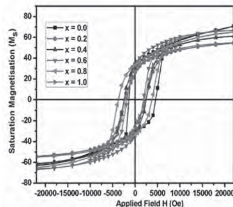
Fig.1 M-H loops of for pure BaM and Cobalt substituted BaM sintered at 900^\circ\text{C} .
