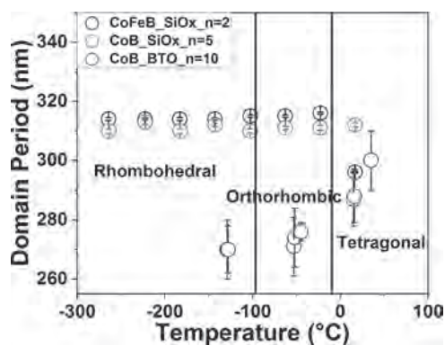
Fig.1. Temperature dependence of the magnetic domain period for the multilayer Pt/Co(Fe)B/Ir n=2,5,10 grown on SiO x and BTO substrates. The labels 'Rhomboidal' etc [3], refer to the structure of the BTO substrate at the given temperature.
