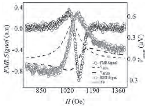
Fig. 1 : FMR spectra and spin pumping voltage ( V_{\text{meas}} ) measured at = 39^\circ with applied dc magnetic field ( H ).
