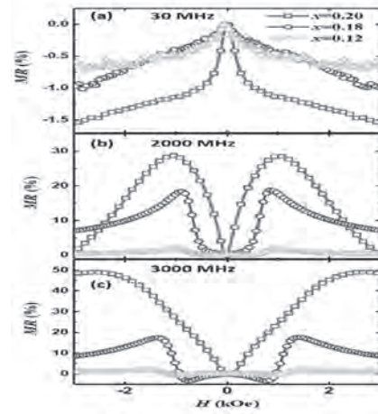
Fig. 1. Ac MR of \text{La}_{1-x}\text{Sr}_x\text{MnO}_3 for x = 0.20 (squares), 0.18 (circles), and 0.12 (triangles) with ac frequencies of (a) 30 MHz, (b) 2000 MHz and (c) 3000 MHz.
