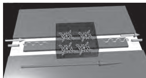
Fig. 1: Pictorial sketch of the coplanar resonator with a VO(TPP) crystal on it. Green arrows represent the microwave pulses, while the red arrow represents the applied static magnetic field. Yellow cylinders are the tunable coupling antennas.
