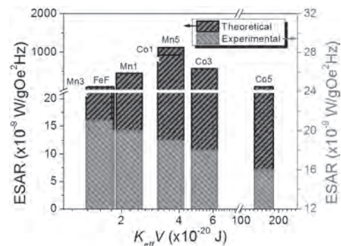
Fig. 2. ESAR of Mn and Co-doped \text{Fe}_3\text{O}_4 as a function of magnetic anisotropy energy.
