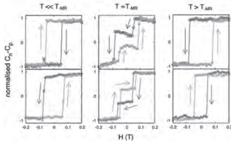
Element specific XMCD hysteresis loops of a Ni 3 Pt(8.5nm)/Ir(0.5nm)/Co(1nm) SFM recorded at temperatures T < T_{\text{MR}} (~200K), T \sim T_{\text{MR}} (~220K) and T > T_{\text{MR}} (~250K), with Co (blue) loops shown on top and Ni (red) shown below. Arrows show the direction of the field sweep.
