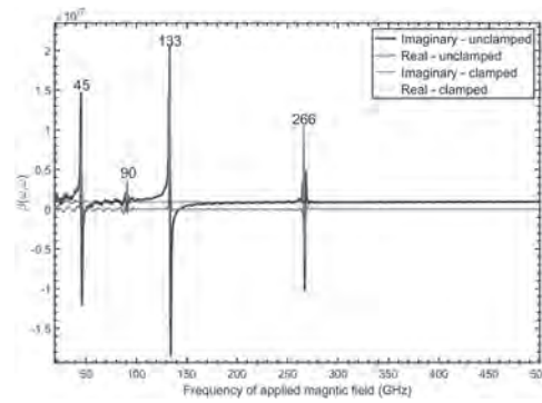
Fig. 2. \beta(\omega, \omega) , vs. \omega
