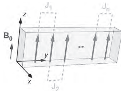
Fig. 1 Illustration of the geometry. The value of the exchange coupling constant increases as one moves to the right.
