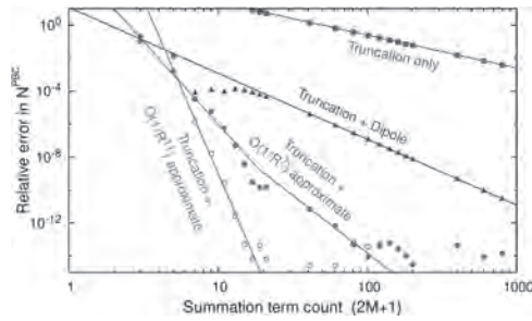
Relative error in N^{\text{PBC}} for a sample with discretization cell geometry 2 \times 3 \times 1 and a 1D periodic window width W=20 . The top curve (filled squares) is error when the PBC sum is truncated at \pm M . The lower curves show error improvement using higher order approximates.
