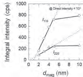
Fig. 2. Integral intensity of L1_0 FePt phase derived from in-plane XRD plotted against d_{\text{mag}} for the typical granular film with SnO.
