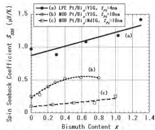
Fig. 2. The dependence of S_{\text{SSE}} on Bi-content (a) Our measurements, (b) Ishida, 2 (c) Asada et al. 4
