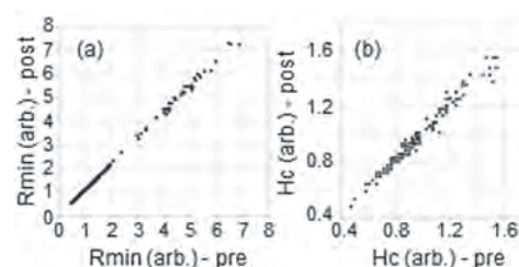
Fig. 2. pMTJ resistance R_{min} (a) and magnetic field switching coercivity H_c (b) measured post vs. pre exposure to 7 Mrad(Si) gamma radiation.
