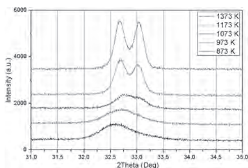
Fig.1. The variation of the main XRD peak of \text{LaCo}_{0.5}\text{Fe}_{0.5}\text{O}_3 with varying sintering temperature.
