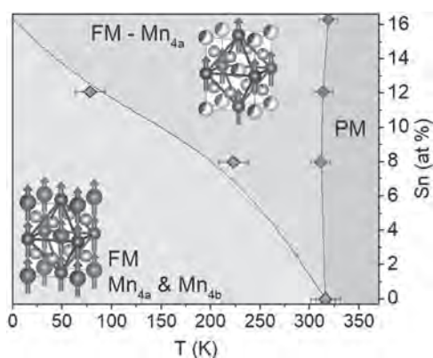
Fig. 2: Magnetic phase diagram of \text{Ni}_{48}\text{Mn}_{36}\text{In}_{16-x}\text{Sn}_x compounds.
