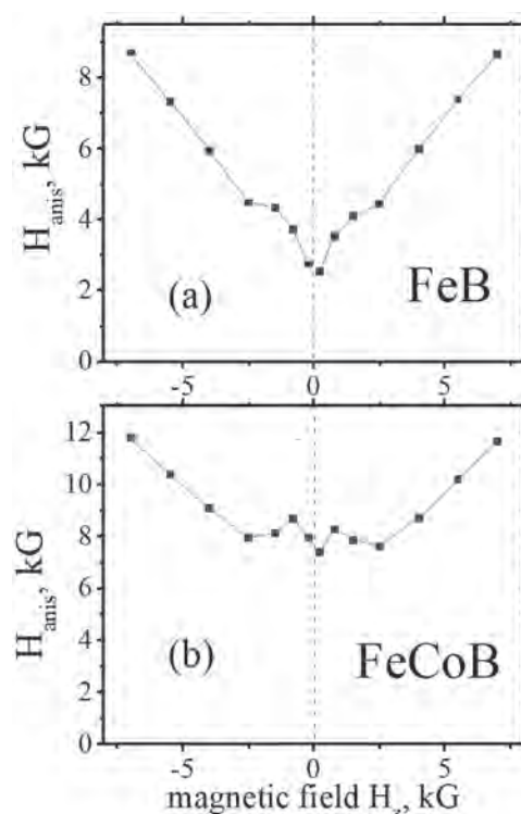
Fig.1 Anisotropy field H_{\text{anis}} as a function of external magnetic field H_z applied perpendicularly to interface and along the magnetization. (a) magnetically-soft FeB nanomagnet. (b) magnetically-harder FeCoB nanomagnet
