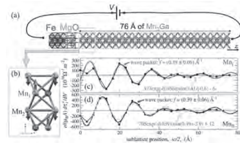
Fig. 1: (a) Schematic of the Fe/MgO/ \text{Mn}_3\text{Ga} junction studied, (b) the unit cell of tetragonal \text{Mn}_3\text{Ga} depicting also the magnetic moments localised on the \text{Mn}_1 and \text{Mn}_2 magnetic sublattices. Shown in the graphs are atomically-resolved linear-response STT on \text{Mn}_1 and \text{Mn}_2 , panels (c,d) respectively, starting from the MgO interface. The structures are periodic in the x-y plane.
