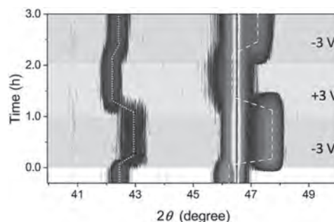
In situ XRD of SCFO- \text{Co}_3\text{O}_4 nanocomposite around the (002) peak of \text{SrTiO}_3 . The line on the left corresponds to \text{Co}_3\text{O}_4 , and the line on the right corresponds to SCFO.
