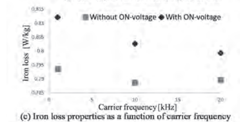
(c) Iron loss properties as a function of carrier frequency
