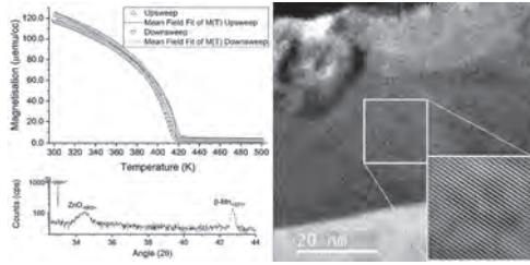
Fig.1. (a) M(T) of Co 47 Zn 53 alloy, annealed at 400 °C for 48 hrs; (b) XRD of sample (a), identifying the (221) β-Mn phase; (c) TEM image of crystalline order in a Zn-rich sample under the same preparation conditions.
