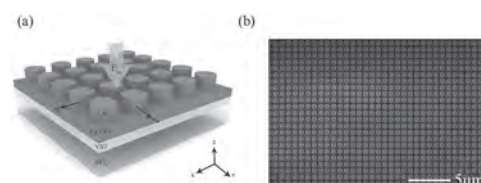
Fig. 1 (a) Schematic diagram of the metasurface (b) Scanning electron microscope image of a fabricated device
