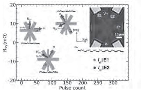
The R_{xy} signal during current pulsing along the hematite E1 (red) and E2 (blue) easy axes at H_{\text{IP}} which rotates n along the easy axes, and corresponding orientations of n indicated on the device schematic. Device micrograph and pulsing directions are shown in the inset.
