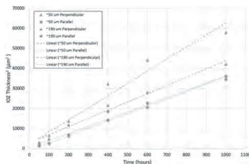
Fig.1 IOZ growth at 500^\circ\text{C} , varying with growth direction in respect to crystallographic c -axis and grain size
