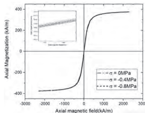
Modeled hysteresis loop for a point in the MRE under compressive stresses
