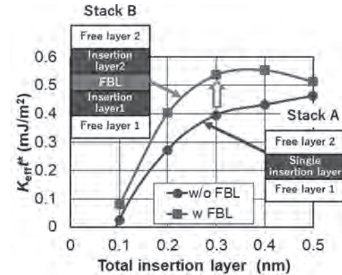
Fig.2 total non-magnetic insertion layer thickness dependence of K_{\text{eff}}^*
