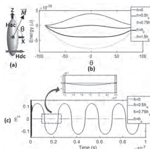
Figure 1: (a) Nanomagnet with AC field along the easy (Z) axis and dc bias field along the hard axis (X). (b) Energy plot as a function of \theta and for various DC fields. (c) Non-thermal oscillation for different values of DC fields.
