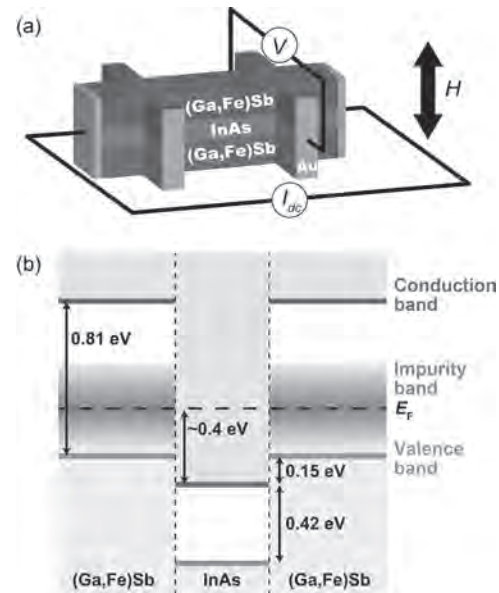
Fig. 1. (a) Schematic device structure and measurement configuration of the Hall bar devices with size of 100 \times 400 \mu\text{m}^2 . (b) Schematic band alignment. The Fermi level E_F is pinned at 0.2 – 0.3 eV above the valence band top of the (Ga,Fe)Sb 5 .
