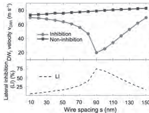
(top) DWI velocity v_{DW} under inhibition (red circles) and non-inhibition (blue squares) conditions; (bottom) lateral inhibition LI as a function of spacing between DW tracks, s .
