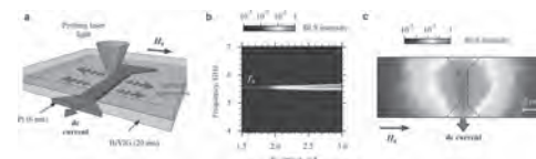
Fig. 2 (a) Experimental layout. (b) Measured spectra of current-induced magnetization auto-oscillations. (c) Measured spatial map of the spin-wave intensity.
