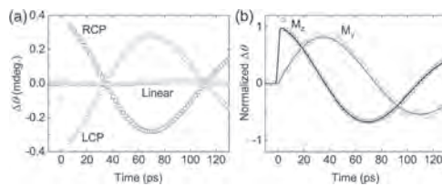
Figure 2: Optical spin-orbit torque. (a) The measured dynamics of the z-component of Co magnetization in the sap/Pt(5)/Co(3)/MgO(3) sample driven by pump pulse, incident on the substrate side, with right circular polarization (RCP) (black squares), left circular polarization (LCP) (red circles), and linear polarization (blue triangles). Given the negative value of the static Kerr rotation of Co (Supplementary Note 6), positive/negative \Delta\theta of (a) indicates -z/+z tilting of magnetization. (b) The comparison of the M_z (black squares) and M_y (red circles) dynamics of Co in the sap/Pt(5)/Co(3)/MgO(3) sample. The black and red lines are fitting with cosine and sine functions, respectively [5].
