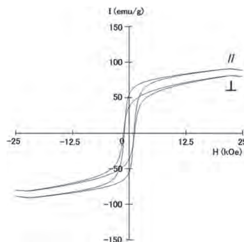
Fig.1 Hysteresis loops of the hot-deformed \text{Sm}(\text{Fe,Ti})_{12} magnets.
