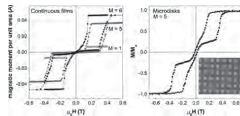
Figure 1. Room temperature out-of-plane hysteresis loops of SAF multistacks.
