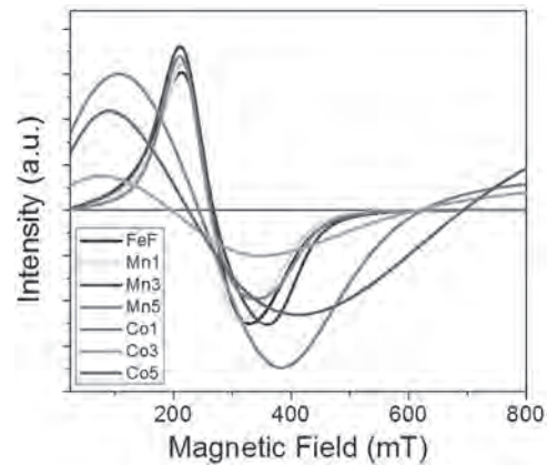
Fig. 1. ESR spectra of Mn and Co-doped \text{Fe}_3\text{O}_4 .
