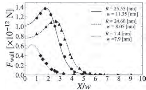
Fig. 2 The simulation (dots) and analytical results (curves) of the forces between 3 different skyrmions and walls. The curves are symmetric across X=0 .
