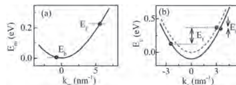
Fig.2 (a) Magnon dispersion (b) Electron dispersion outside the spin chain (dashed curve) and majority spin dispersion in the spin chain (solid curve). The energies E_f , E_b of forward- and the backward-propagating magnon groups are indicated.
