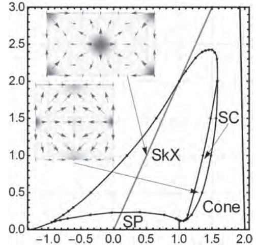
Zero temperature phase diagram of AFM with DMI. The axes correspond to the dimensionless staggered magnetic field and dimensionless effective anisotropy. The gray line separates the aligned and the tilted regions of the FM phase. This phase is taken over by the hexagonal skyrmion lattice (SkX), spiral (SP), cone phase, and the square crystal of vortices and antivortices (SC). The upper inset shows a hexagonal lattice unit cell with a skyrmion in the center. The lower inset shows a square crystal unit cell with AFM antimeron in the center. Red and yellow correspond to positive topological charge density and blue corresponds to the negative topological charge density.
