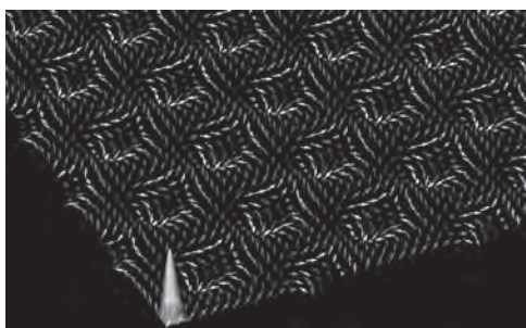
Fig. 1. Antiskyrmion crystals support topological magnonic corner states. Magnetic texture of an antiskyrmion crystal in the vicinity of a sample corner. Fractional antiskyrmions that self-assemble along the sample edge allow the emergence of a topological magnonic state whose probability amplitude (depicted in yellow) is corner-localized.
