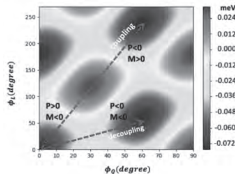
Energy landscape with \Phi_0 and \Phi_L as coordinates, where Q is fixed at 0.33 \text{ \AA} .
