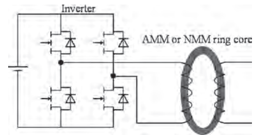
Schematic of ring test under PWM inverter excitation.
