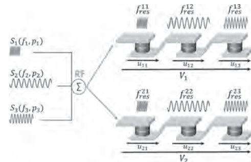
Fig.2 several signals are summed and send to different chains of resonators to implement a MAC operation.
