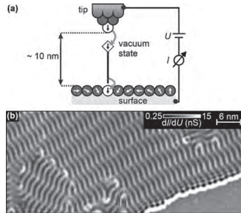
Figure: (a) Schematic sketch of the experimental approach. The net spin-polarized tunnel current flowing from the scanning probe tip via the vacuum states to the sample is recorded and analyzed. Achievable tip-sample distances are indicated. (b) Magnetic map of an ultrathin Fe film grown on Ir(111) exhibiting spin spirals, imaged via spin-polarized resonant tunnelling.
