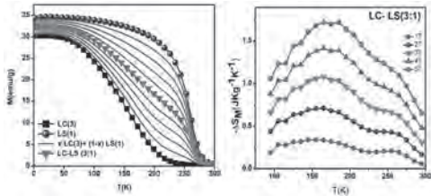
Fig. 1 (a) Magnetization vs. Temperature curve (b) Magnetic entropy change ( -\Delta S_M ) vs. temperature at different applied fields for LC-LS(3:1) samples.
