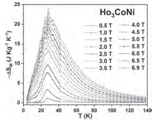
Fig. 1. Magnetic entropy change -\Delta S_M for \mu_0\Delta H from 0.5 T to 6.9 T for \text{Ho}_3\text{CoNi}
