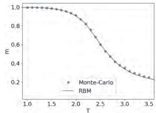
Fig. 2. Magnetization in 2D ferromagnetic Ising model
