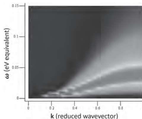
Fig. 2. An example magnon dispersion. Spatial symmetry is imposed by the perturbing field, such that magnons are created at the centre of the lattice and propagate outwards
