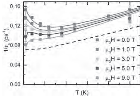
Fig. 2. 1/\tau_s as a function of temperature, for different magnetic fields. The dashed line is an MI-free estimate of 1/\tau_s .
