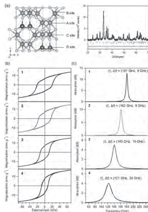
Figure 1. (a) Crystal structure of \epsilon -( \text{TiCo} ) _{0.033}\text{Fe}_{1.934}\text{O}_3 and XRD pattern of 3. (b) M-H curves at 300 K and (c) millimetre wave absorption spectra.
