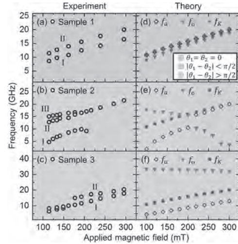
Fig.1. Dependence of the frequency on the applied magnetic field for the different modes. (a)-(c) Experimental data: the different precessional modes are indicated with Roman numbers. (d)-(f) Theoretical data: f_a , f_o and f_K are the frequency of the acoustic mode, optical mode, and the FMR mode for a 7.5 nm CoFeB film. The three different background colors indicate the three field regions given in the inset of (d).
