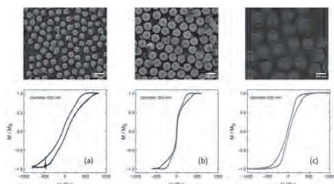
SEM images (upper panel) together with corresponding hysteresis loops (lower panel) for \text{Fe}_{70}\text{Pd}_{30} nanodisks having 30 nm thickness and diameter: (a) 250 nm; (b) 350 nm and (c) 500 nm.
