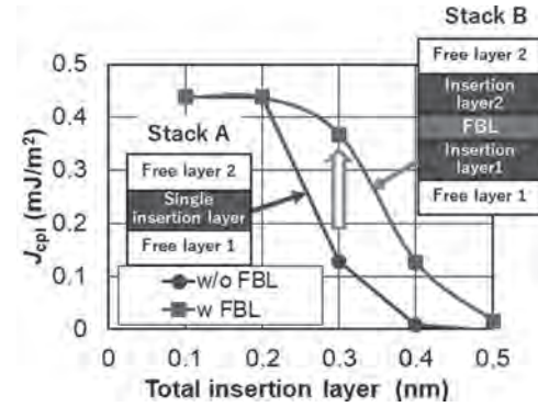
Fig.1 total non-magnetic insertion layer thickness dependence of J_{\text{cpl}}
