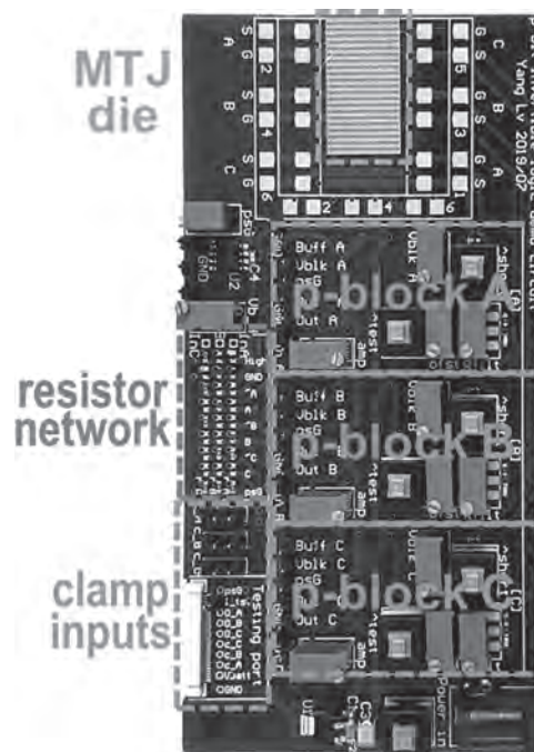
Fig. 1. Photograph of p-bit and PSL demonstration hardware. Note that a 'p-block' refers to a specific hardware implementation of a p-bit.
