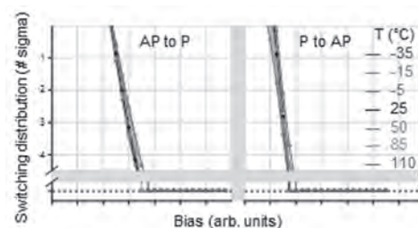
Fig. 1. STT write distributions in both transition directions in a 1Gb die measured across temperatures from -35°C to 110°C.
