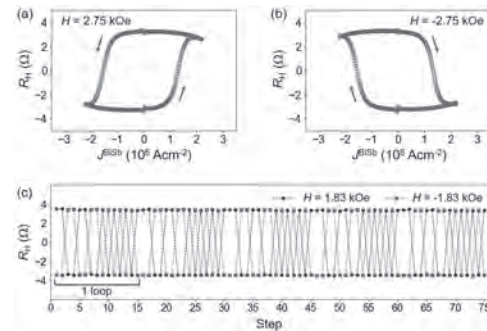
Fig. 2 (a) (b) SOT switching by DC currents at +2.75 kOe and -2.75 kOe, respectively. (c) Robust switching by 75 consecutive pulses at \pm 1.83 \text{ kOe} ( J^{BiSb} = 4.4 \times 10^6 \text{ Acm}^{-2} , t_{pulse} = 100 \mu\text{s} ).
