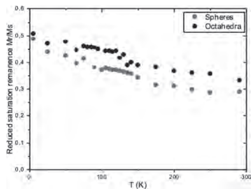
Figure 1. Temperature dependence of the reduced saturation remanence measured in the spherical and octahedral NPs
