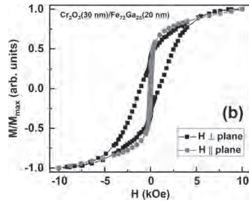
(b) \text{Cr}_2\text{O}_3(30 \text{ nm})/\text{Fe}_{72}\text{Ga}_{28}(20 \text{ nm}) .
