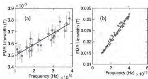
Figure 2. Out-of-plane FMR linewidth versus frequency for (a) (25nm) BiYIG/SGGG (b)BiYIG (15.5nm)/TmIG(5.6nm)/NGG film
