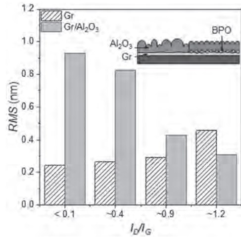
Roughness of graphene before (hatched) and after (grey) Al evaporation, creating an Al 2 O 3 layer, versus I_D/I_G ratio. Inset: Schematic of roughness difference with and without molecules on top of graphene.
