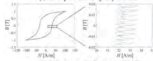
(b) BH loop at carrier frequency of 20 kHz
