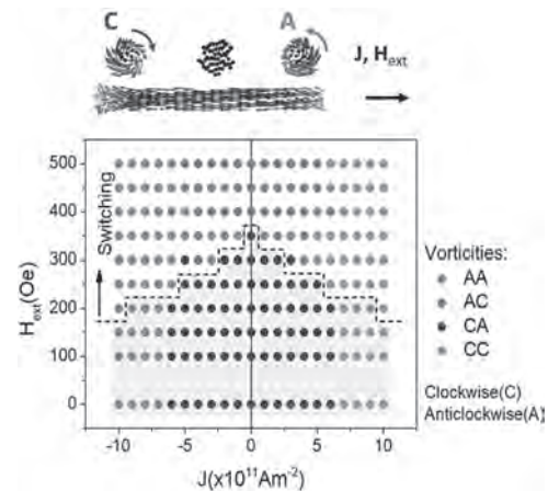
Fig.1. Diagram of magnetization vortex states: Vorticities of the vortex (or curling) structures at the ends of the nanowire in the final state obtained after the application of magnetic field, H_{\text{ext}} , and current density, J . C(A) stands for Clockwise (Anticlockwise) vorticity as indicated in the upper sketch. The threshold for the axial component switching field is indicated by the dashed line. No magnetization switching occurs below this line (yellow-shaded region).
