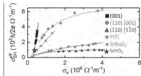
Comparison of SHC with the electrical conductivity of various planes and directions of IrO 2 with other materials such as Pt-Ti alloys, SrRuO 3 and SrIrO 3
