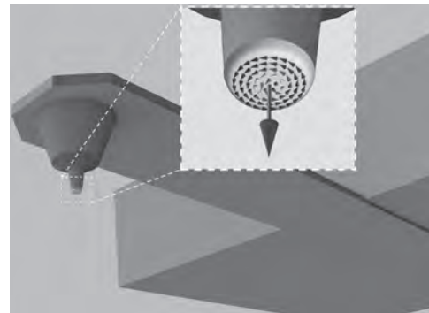
Schematic sketch of VC MFM tip. The magnetically soft disk from permalloy is deposited on the apex of Si tip. In the center of the disk, small vortex core is formed creating well localized out-of-plane magnetic moment (shown as big red arrow).
