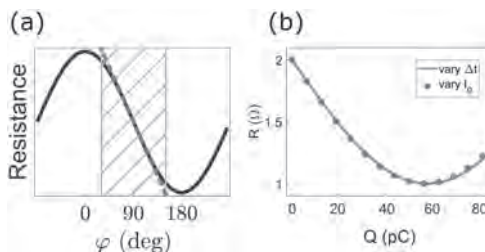
Fig.1 (a) Expected angular range of nearly ideal memristive behaviors. (b) Dependence of resistance variation on the total charge Q = I_0 \cdot \Delta t of the current pulses with varied amplitude I_0 at fixed duration \Delta t and varied \Delta t at fixed I_0 .
