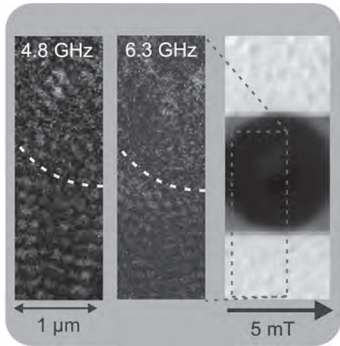
Fig. 2: Spin waves in YIG (TR-STXM) [8].
