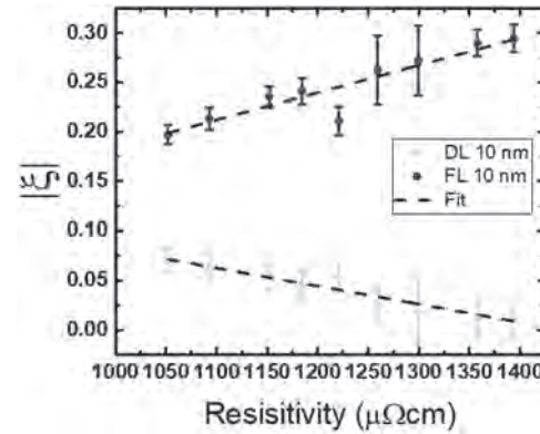
Fig. 2. Relation between magnitude DL and FL torque efficiencies and the resistivity of the 10 nm Ru 2 Sn 3 sample.
