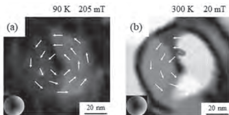
Fig.2 LTEM images of single skyrmions of \text{Fe}_{1.68}\text{Pd}_{0.32}\text{Mo}_3\text{N} films. (a) at 90 K (b) at 300 K.
