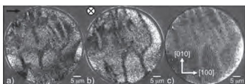
(a) In-plane SPMEEM, (b) out-of-plane SPMEEM, and (c) ultraviolet magnetic field dichroism images from the surface of \text{Fe}_3\text{O}_4(100) . Field of view: 50 \mu\text{m} .
