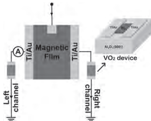
Schematics of the structure of our magnetic logic-memory device. Magnetization of magnetic film and the channel current are logic input and output, respectively. The Schematic of a two-terminal VO 2 device is indicated in the inset.
