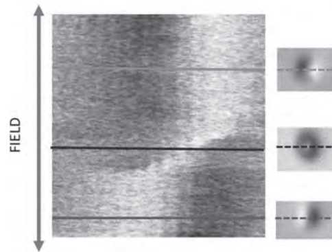
Nonstandard MFM image of a Py nanodot (height ~30 nm). With this method, we can study the magnetization process of a single particle.
