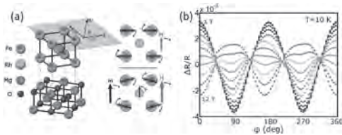
(a) Schematic of FeRh grown on MgO. In our main results, the current is aligned along the [100] direction as indicated and the external field is allowed to rotate in the plane of the FeRh. The right schematic shows how increasing the external induces magnetization ( m ) in the FeRh from by tilting the magnetic moments. The curved arrows give a sense of how the moment structure and the external field rotate within the plane. (b) The AMR is shown as a function of the in-plane angle for applied fields between 1 T and 12 T. At low fields, the AMR is mainly two-fold but a four-fold structure becomes apparent as the field increases. At the highest fields (10-12 T) the two-fold AMR signal clearly changes sign.
