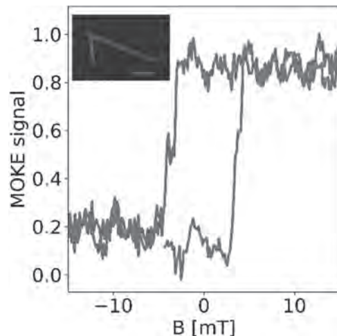
Fig. 2: Dark-field MOKE measurements of a 3D nanowire deposited with FEBID. Scale bar is 1µm.
