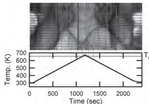
Fig.1 (top) A Y-time slice of a pseudo 3D image exhibiting temperature-dependent domain structure and (bottom) a temperature-time profile. Horizontal black and white stripes with a constant period are DW images, while the broad black bands bending along time axis are non-magnetic contrast (bend contours).
