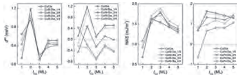
Calculated DMI and magnetic anisotropy energy as functions of Co atomic layer number and doping concentration at the Co/diamond interfaces.
