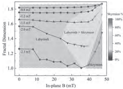
Fractal dimension ( D_f ) extracted from MOKE imaging vs the in-plane magnetic field ( B_{||} ). With proportion of Skyrmions indicated by the colour scale. For each curve, we start with different initial out-of-plane magnetic fields ( B_{\perp} ), and then ramp B_{||} from 0 mT to 47.3 mT.
