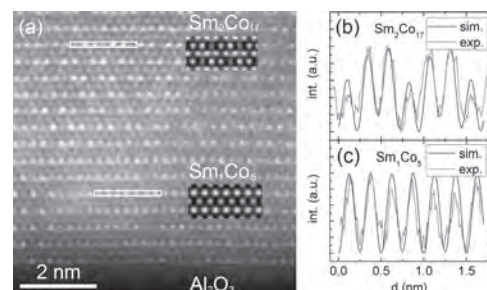
Fig. 2: Thin film nanocomposite of Sm-Co system comprising of \text{SmCo}_5 and \text{Sm}_2\text{Co}_{17} phases.
