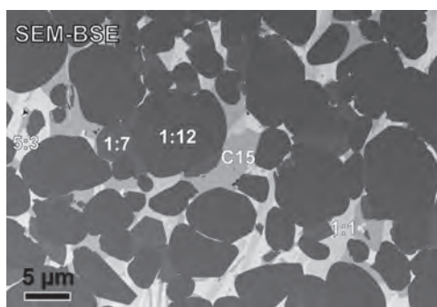
Fig. 2 BSE-SEM micrograph of Sm-rich Ga-containing alloy showing \text{Sm}_5\text{Ga}_3 (5:3), \text{SmGa} (1:1) and \text{Sm}(\text{Fe},\text{Co},\text{Ga})_2 (C15) intergranular phases in bright contrast.
