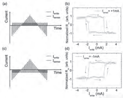
Figure 2. (a,c) Measurement sequence for the switching experiment and (b,d) Current-induced DL-SOT switching results of a W(3)/CoFeB(1.8) Hall-bar sample with opposite sense currents I_{sense} = +1 mA and I_{sense} = -1 mA.
