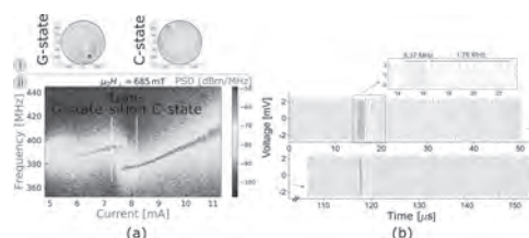
Micromagnetic representation of gyrotropic and C-state with and without vortex core inside the nanodisk, resp (a.i). A C-shaped in-plane magnetization characterizes the C-state. (a.ii) Measurement of the two distinct states: The transition is triggered by the applied dc current. (b) Measurement of the transition between the two states via a heterodyne technique: Switching between the states is stochastic.
