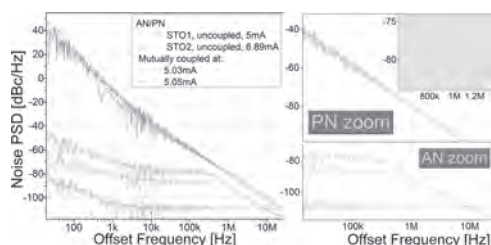
(a) Noise power spectral density of two vortex based spin torque nano oscillators alone (green, blue) and synchronized at different conditions (gray, reddish): The coherence improvement at synchronization leads to a decreased phase noise (PN). However, a significantly increased amplitude noise (AN) is observed.
