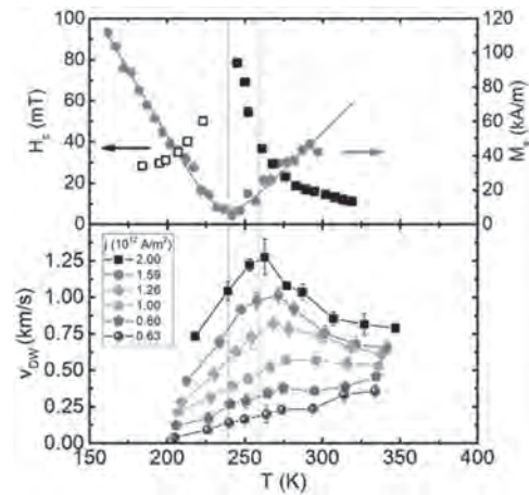
Coercivity ( H_c ), magnetization ( M_s ) as a function of temperature ( T ) and domain wall velocity ( v_{DW} ) as a function of temperature ( T ) for various current densities ( j ) in Pt/Gd 44 Co 56 /TaOx. The tan vertical line indicates magnetic compensation, while the green vertical line indicates angular momentum compensation.
