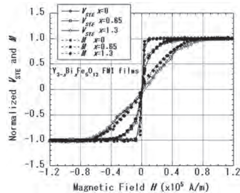
Fig. 1. Comparison between the normalized V_{\text{STE}} - H and M - H curves: l_d=5\text{ mm} ; t_{\text{Pt}}=4\text{ nm} .
