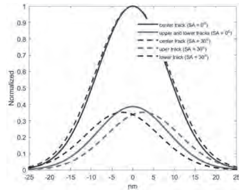
Fig. 1: The impulse responses of the upper, center, and lower tracks for various SAs.
