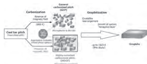
Fig. 1. Preparation processes of graphite.
