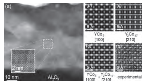
Fig. 1: Thin film nanocomposite of Y-Co system made up of \text{YCo}_5 and \text{Y}_2\text{Co}_{17} phases.
