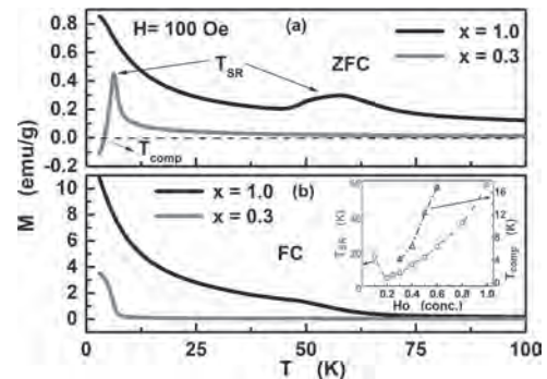
(a) M_{\text{ZFC}}(T) , (b) M_{\text{FC}}(T) . Inset in (b): T_{\text{SR}}(x) , T_{\text{comp}}(x)
