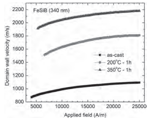
Fig. 1. Domain wall velocity vs. applied field for an FeSiB amorphous submicron wire, with the annealing temperature as a parameter.
