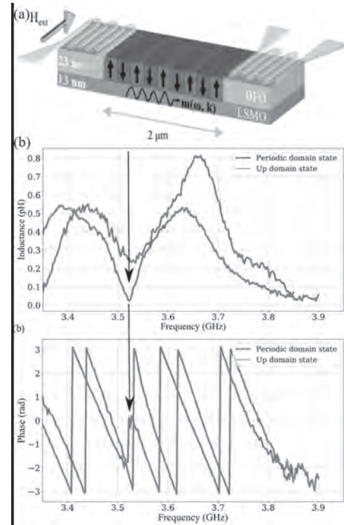
Fig. 1: (a) Experimental setup with periodic BFO domains (b) Evidence for the bandgap for the BFO/LSMO heterostructure with periodic domains in the BFO for the transmission amplitude of the inductance (top) and the corresponding phase response (bottom)
