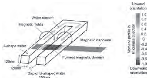
Fig.1 LLG simulation of magnetic domain formation in a magnetic nanowire by using a U-shaped writer.
