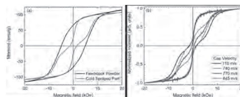
Figure 1: (a) Room temperature M-H loops for NdFeB, showing formation of a secondary phase due to particle damage. (b) Analysis of link between gas velocity in particle damage shows that reducing kinetic energy improves magnetic performance.
