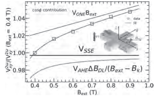
\cos\phi_B contribution of the measured second harmonic Hall voltage as a function of an externally applied in-plane field for a CGT/Pt sample. The data are fit to spin-Seebeck (black), ordinary Nernst effect (red) and damping-like torque (red) contributions. The green and red curves are offset by V_{SSE} for comparison. After subtraction of the thermoelectric signals, anti-damping spin torque efficiency of \xi_{DL} = 0.25 \pm 0.09 is obtained.
