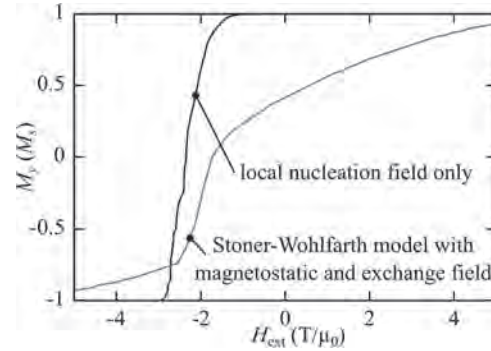
Fig. 2: By applying the Stoner-Wohlfarth model and including the magnetostatic and the exchange field, a realistic hysteresis curve of a 180 \times 120 \mu\text{m}^2 thin film sample was calculated.
