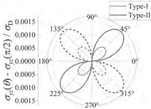
Fig. 2. Transverse magnetoconductivities of Type-I and Type-II Weyl semimetals.
