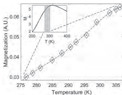
Fig. 1: 9.5 nm MNP
