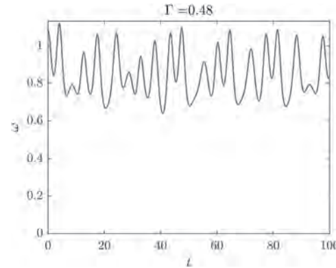
Magnitude of angular velocity \omega of the Néel order, which is proportional to the spin-pumping signal. The peaks and valleys of the signal appear with no pattern.
