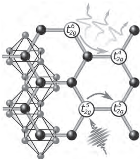
Fig. 2) \alpha -RuCl 3 's honeycomb lattice. The lower process shows the photogeneration of a holon-doublon pair. The upper process shows the subsequent multimagnon emission by holon-doublon recombination, which drives the system into a nonequilibrium quasistationary spin disordered state.
