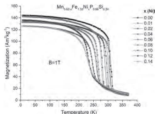
Fig. 2. Temperature dependence of the magnetization in the magnetic field of 1 T for \text{Mn}_{0.62-x}\text{Fe}_{1.33}\text{Ni}_x\text{P}_{0.66}\text{Si}_{0.34} upon heating and cooling.
