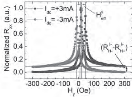
Figure 1. Representative shifted AMR loops measured from a W(3)/CoFeB(1.8) sample with dc current I_{dc} = \pm 3 mA.
