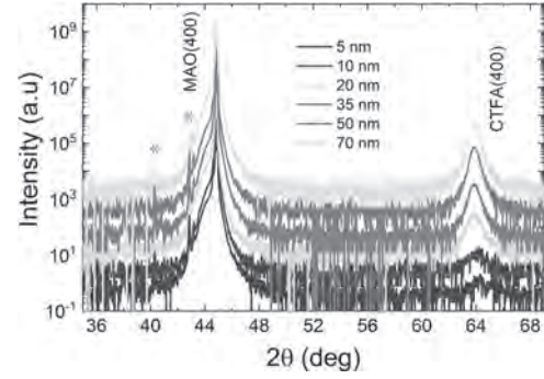
Fig. 1. 2θ-ω XRD (Cu X-ray source) scan of epitaxial \text{Co}_{1.5}\text{Ti}_{0.5}\text{FeAl} thin films (vertically offset for clarity) grown on MAO (100) single crystal substrates. Asterisks (*) indicate substrate peaks.
