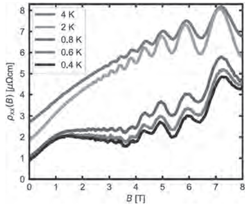
Fig.1 : Shubnikov-de-Haas oscillation observed in the \text{CeTe}_3 thin film.
