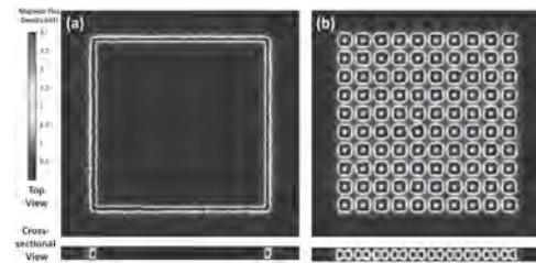
Fig. 2: Proposed permanent magnet integration strategy. A thin film (a) produces magnetic field only at the edges whereas the flux density (or gradient) can be significantly improved by micro-patterning (b) of the magnet. Magnetic flux intensity variation is shown by the color distribution.
