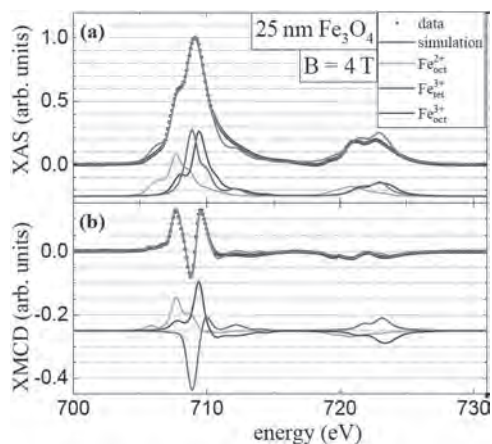
Fig. 1: (a) XAS and (b) XMCD spectrum at the Fe L 2,3 edge for a 25 nm Fe 3 O 4 thin film, taken at 4T external magnetic field, at room temperature and in TEY mode. Black dots are data points; green, red and blue spectra are multiplet calculations for the three cation species of Fe 3 O 4 , the grey line is their sum.
