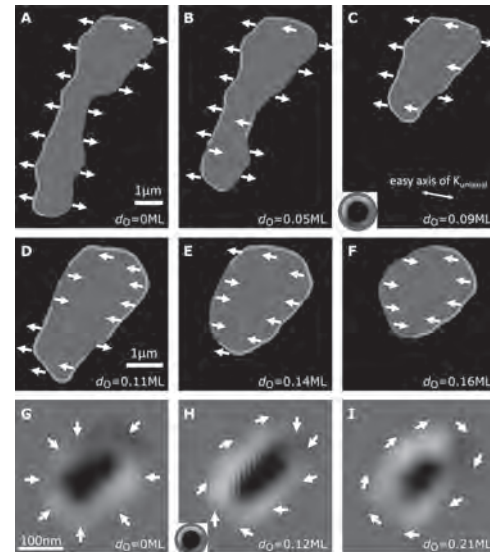
Figure 1 Oxygen-assisted chirality modification at room temperature. (A-F) SPLEEM images of a magnetic bubble in perpendicularly magnetized thin films with increasing oxygen coverage (labeled in each panel), showing a complete chirality transition from left-handed (panel A) to achiral (panel D) to right-handed (panel F). Color wheel and white arrows show in-plane magnetization directions. Grey/black regions show out-of-plane components of the magnetization pointing down (-z) or up (+z). (G) Compound SPLEEM image of a left-handed Néel-type skyrmion in a perpendicularly magnetized thin film system. (H-I) The Néel-type skyrmion in panel G evolves into a skyrmion with tilted wall and finally a Bloch-type skyrmion upon oxygen chemisorption.
