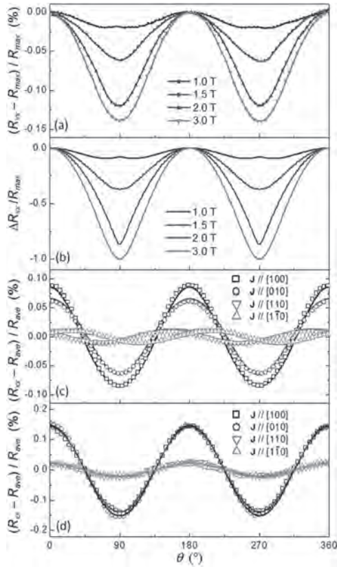
Fig.2 Resistance vs. angle between field and current directions, (a) for 10 nm CuMnAs, with current along the [010] direction and H = 1.0, 1.5, 2.0 and 3.0 T at 4 K. (b) Calculated AMR for uniaxial antiferromagnet with a Gaussian distribution of spin-flop fields centered on 1.6 T. (c,d) for 10 and 50 nm CuMnAs, with magnetic field 5 T at 4 K. The lines are fitting results.
