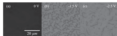
Fig. 2: MOKE images of domain structures of MgO/ Mn 2 CoAl/ Pd trilayers captured with H_z = -1 mT at 0, -1.5, -2.5 V, respectively.
