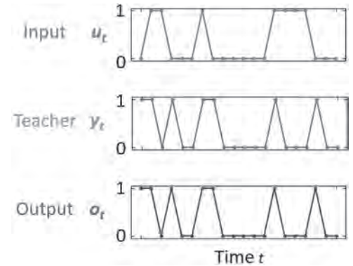
Fig. 2 An example of input, teacher and output after training. The teacher function is parity check with a time delay = 1 for checking the non-linear computation capacity of the reservoir.
