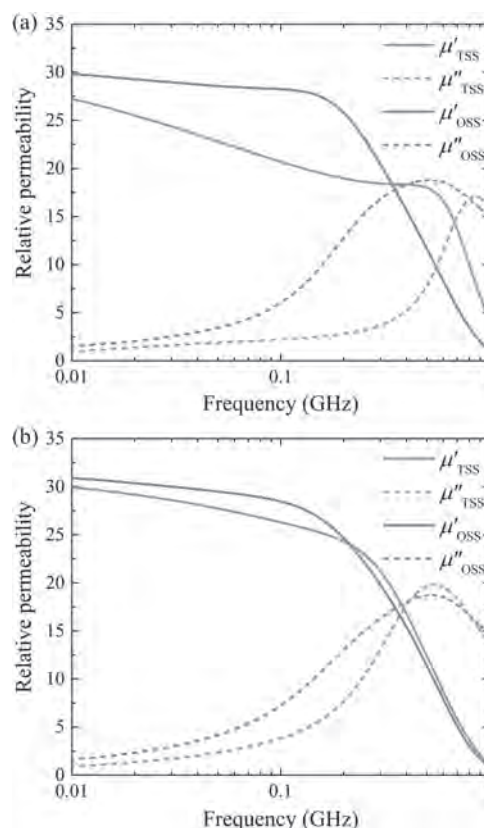
Fig. 2. Relative permeability spectra of \text{BaCo}_{1.2}\text{Ti}_{1.2}\text{Fe}_{9.6}\text{O}_{19} samples sintered by one-step sintering and two-step sintering with different densities of (a) 88.8% and (b) 95.4%.
