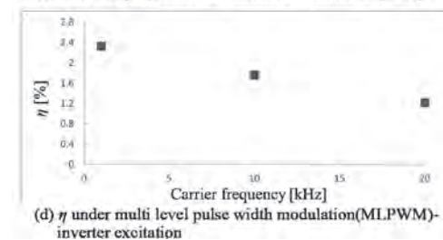
Magnetic properties under MLPWM-inverter excitation.
