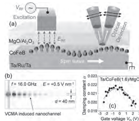
(a) Schematic diagram shows the excitation of propagating spin waves by VCMA and detection by magneto-optical Kerr effect (MOKE). (b) Simulation result shows the propagation of SW through a VCMA induced nanochannel. (c) Nonlinear variation of damping constant in ultrathin CoFeB film by electric field.
