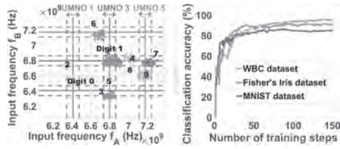
Fig. 2: (a) Synchronization pattern of five UMNOs to classify images for 10 digits (0–9) in MNIST (b) Classification accuracy for MNIST, Iris and WBC datasets
