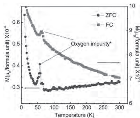
Magnetization versus temperature curve obtained under ZFC and FC conditions
