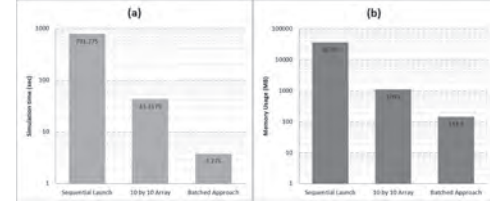
Fig.2: (a) Computational time and (b) memory consumption.
