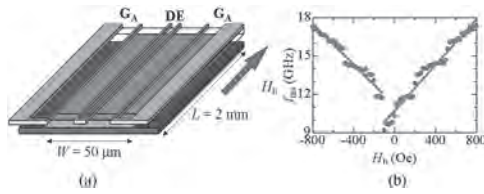
Fig. 1. (a) Schematic of a designed phase comparator, (b) The dependence of SSWR on H_b .
