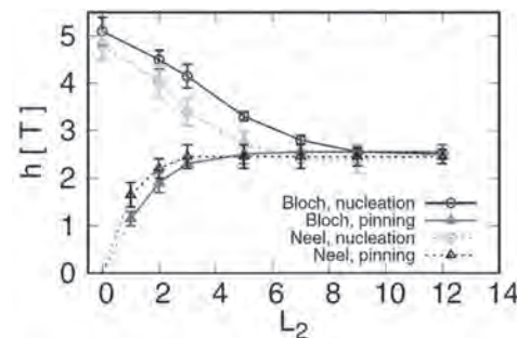
L2 (the thickness of the soft magnet) dependence of the nucleation and pinning fields of the Nd magnet model.
