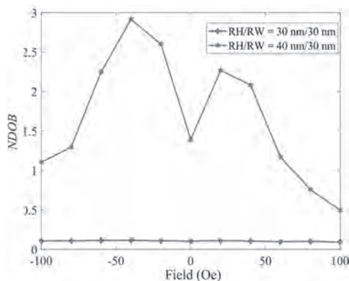
Fig. 1 Macrospin model: noise in the device operation band ( NDOB ) vs. the external field - comparison between no shape anisotropy and high shape anisotropy readers with the same bias field (= 800 Oe). The model does not include shields, so the external field magnitude is much lower than in the experiment (Fig. 2).
