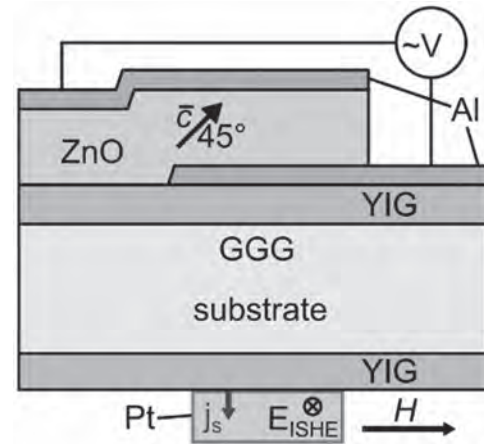
Fig.1. Schematic of hybrid HBAR for acoustic spin pumping. The rf voltage V is applied across the piezoelectric transducer sandwiched between thin-film Al electrodes. The transducer launches and detects a bulk shear acoustic waves, which propagate vertically.
