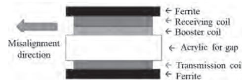
Fig.2 Coil position and displacement direction
