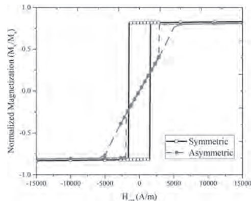
Fig.1: Simulated hysteresis loops for symmetric and asymmetric nanocaps with diameter 100 nm and thickness 10 nm. Square loops account for the magnetization reversal via coherent rotation in symmetric caps. Hysteresis loops for asymmetric caps of diameter 100 nm show negligible remanence and coercivity.
