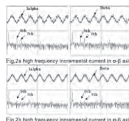
Fig.2b high frequency incremental current in \alpha - \beta axis (the one compensated inductance variation)
