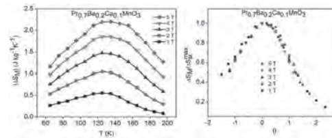
Fig. 1 Temperature dependence of magnetic entropy change for the nanocrystalline \text{Pr}_{0.7}\text{Ba}_{0.2}\text{Ca}_{0.1}\text{MnO}_3 sample at different fields and rescaled magnetic entropy change curves as a function of rescaled temperature.
