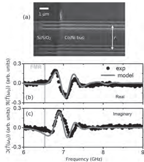
Fig. 1: (a) Colorised scanning electron micrograph of a device with CPW antennas on a Co/Ni multilayer. The scale bar is 1μm. (b) Real and (c) imaginary parts of the experimental transmission parameter and fits.
