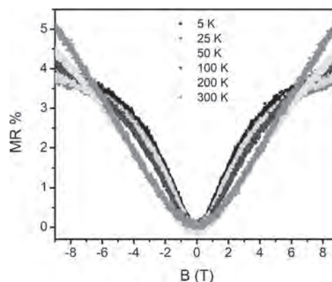
Magnetoresistance (MR) % data for ScPtBi deposited on Si substrate at 200°C.
