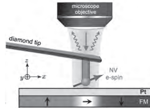
Principle of a scanning-NV magnetometer operating in PL quenching mode.
