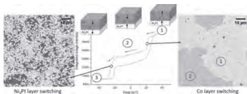
Fig. 1. Wide-field Kerr microscopy of a \text{Ni}_3\text{Pt}/\text{Ir}/\text{Co} structure in a polar geometry. The different domain structure of the Co and \text{Ni}_3\text{Pt} layers allows the magnetization reversal of these layers to be distinguished.
