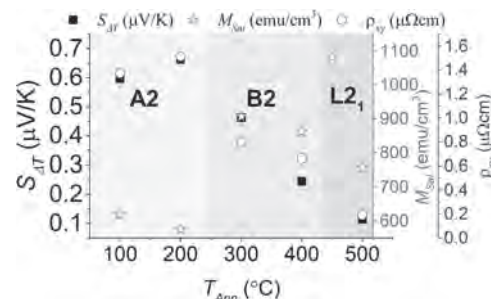
Fig.2 Dependence of ANE ( S_{\text{AT}} ), magnetisation ( M_{\text{sat}} ) and Anomalous Hall resistivity ( \rho_{xy} ) on the ordering of Co 2 MnSi thin films.
