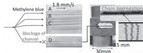
Fig. 1 Blockage of flow channel caused by chain aggregation under homogeneous magnetic field.
