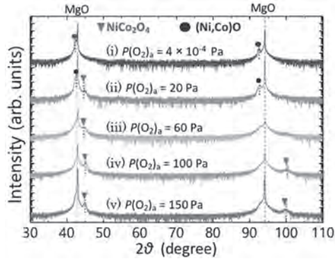
Fig.1 XRD 2\theta/\theta scans of the NCO films with various annealing O_2 pressure.
