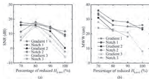
Fig. 1(a) SNRs and 1(b) MWWs for selected parameter sets of the gradient media and notched media.
