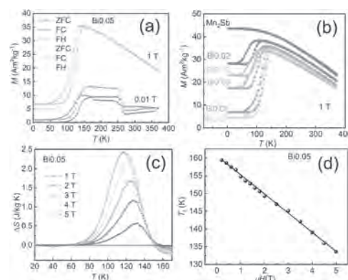
Fig. 1. Temperature dependence of magnetization under the magnetic fields of 0.01 T and 1 T (a) for \text{Bi}_{0.05} and (b) for \text{Mn}_2\text{Sb}_{1-x}\text{Bi}_x ( x = 0.02, 0.05, 0.07, 0.09, 0.15 ) under 1 T. (c) Temperature dependence of entropy change. (d) The critical temperature T_c of AFM-FI as the function of the magnetic field.
