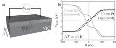
FIG 1: a) In the experimental setup, (Cr, Pt)/YIG samples were subjected to a thermal gradient in the z-direction and a transverse magnetic field which resulted in an observable longitudinal voltage across the samples via LSSE. b) Longitudinal spin Seebeck voltage plotted against magnetic field for a 10 nm Cr sample and a 10 nm Pt sample at a temperature difference of 40 K.
