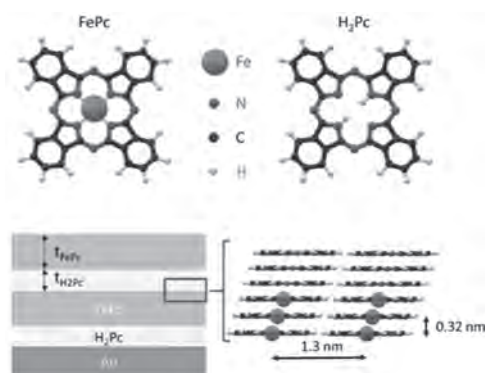
1D Fe chains based in Organic superlattices, and their molecular orientation. Magnetic Iron (II) phthalocyanine ( \text{FeC}_{32}\text{H}_{16}\text{N}_8 ) and weak diamagnetic \text{H}_2 -phthalocyanine ( \text{H}_2\text{C}_{32}\text{H}_{16}\text{N}_8 ) molecules
