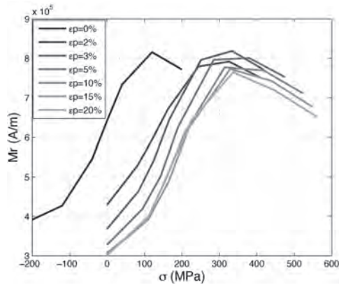
Figure: remanent magnetization M_r as function of stress \sigma for different plastic strain levels \epsilon_p .
