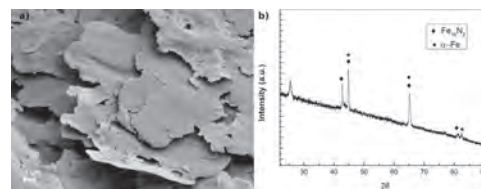
Fig. 1 a) SEM image of Fe_{16}N_2 showing the flake structure. b) XRD measurement of Fe_{16}N_2 flakes, nitrided at 463 K.
