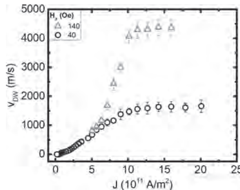
Domain wall velocity v_{DW} as a function of current density J in a low-damping iron garnet/Pt heterostructure for various in-plane fields H_x .
