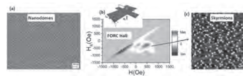
Fig.1: (a) SEM image of the array of nanodomes, (b) FORC Hall diagram of the Pt/Co/Ta multilayer deposited on 100 nm nanodomes, and (c) MFM image of nanodomes showing isolated magnetic skyrmions under an out-of plane magnetic field of 500 Oe.
