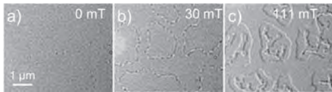
Fig 1. Observation of "Untangling" of Synthetic Antiferromagnet domain walls with application of in-situ perpendicular magnetic field in a Lorentz TEM
