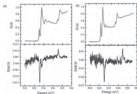
Figure 1. XAS and XMCD spectra of (a) sample S1 and (b) sample S2 at Cu L2,3 edges. All the measurements were performed at 1.7 K under 6 T magnetic field.
