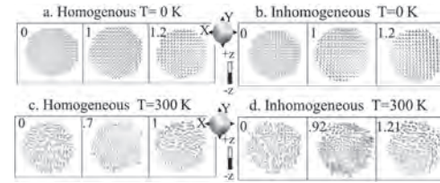
Fig. 1: Micromagnetic spin configurations at different times (shown in left corner in ns) under the SAW excitation applied at t=0 ns for homogeneous anisotropy at a. T=0 K and c. T=300 K and for inhomogeneous anisotropy at b. T=0 K and d. T=300 K.
