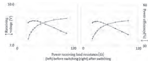
Fig.1 Power receiving load characteristics (left) before switching (right) after switching
