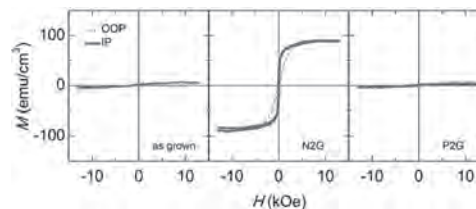
Room temperature magnetic hysteresis loops of as grown, -2V gated, and +2V gated nanocomposite. Magnetization is normalized by the total volume.
