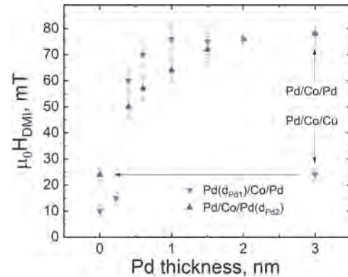
Fig.2. DMI-field as a function of the underlayer and top layer Pd thicknesses
