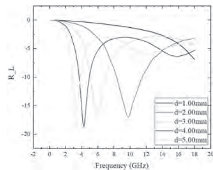
The reflection loss of YFeSi@MOF/paraffin composites.
