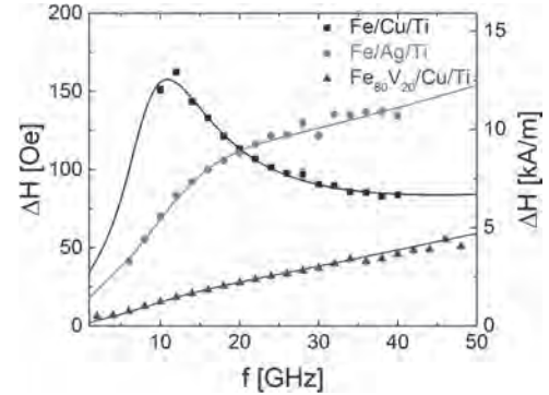
Fig. 2. Linewidth vs. frequency for 10 nm thick Fe/Cu/Ti, Fe/Ag/Ti and \text{Fe}_{80}\text{V}_{20} /Cu/Ti films. Solid curves correspond to fits to the data.
