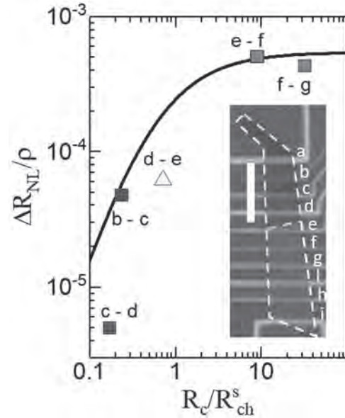
Scaled non-local spin signal as a function of the ratio R_c/R_{ch} . Inset: Optical image of a device with two levels of functionalization, grey and red regions have I_D/I_G ratios of 0.1 and 1.9 respectively. Scale bar is 5 \mu\text{m} .
