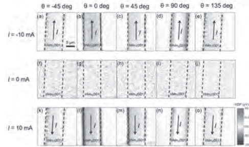
Fig. 1. Two-dimensional helicity dependent photovoltage (HDP) data in (001)-oriented IrMn 3 under various currents. \theta = 0^\circ corresponds to the bias current applied through the [-110] direction in (001)-plane of IrMn 3 . Black dashed lines indicate the edges of the device while black arrows indicate the current direction.
