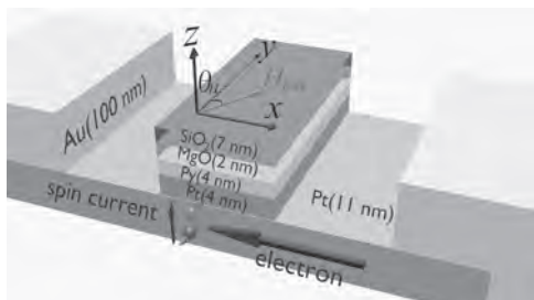
Fig.1. A schematic of device structure for demonstration of current induced magnetization switching.
