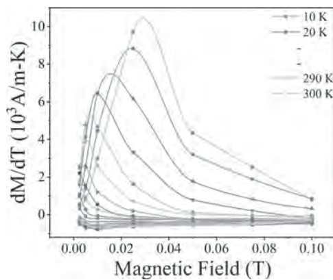
Fig. 1. \delta M/\delta T plots as a function of applied field ( \mu_0 H ) for a TiN/Fe/TiN thin film matrix.
