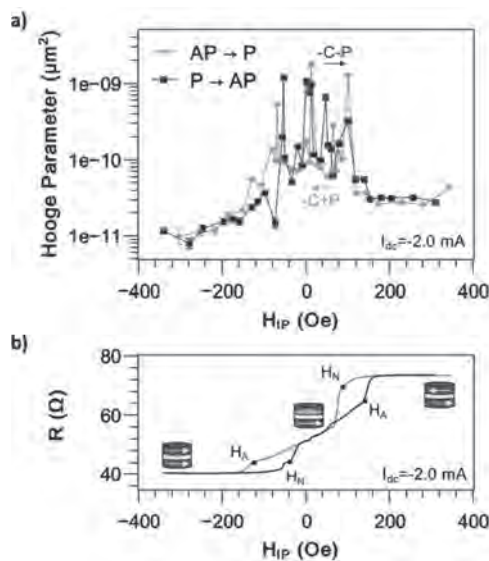
a) Hooke parameter and b) device resistance as an in-plane magnetic field is swept from the parallel to the anti-parallel state and reverse.
